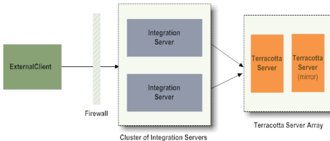
Figure 3. Members of the cluster use caches on the Terracotta Server Array to share data
