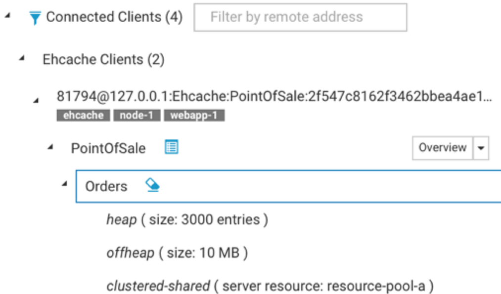
Figure 12. Screenshot: TMC Caching ClientExpanded
