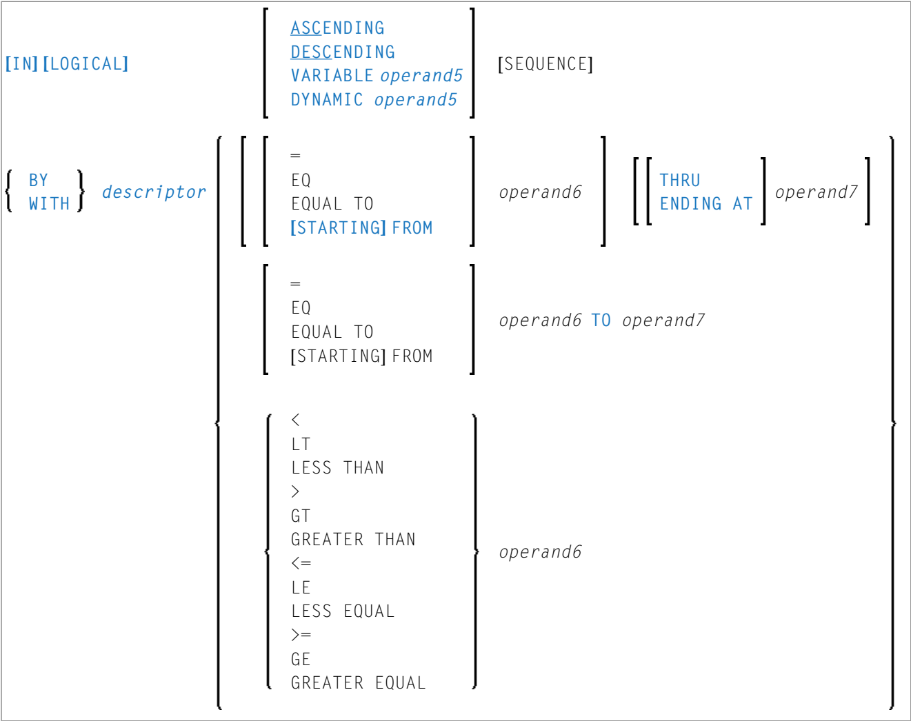
Syntax Option 3: READ BY DESCRIPTOR
