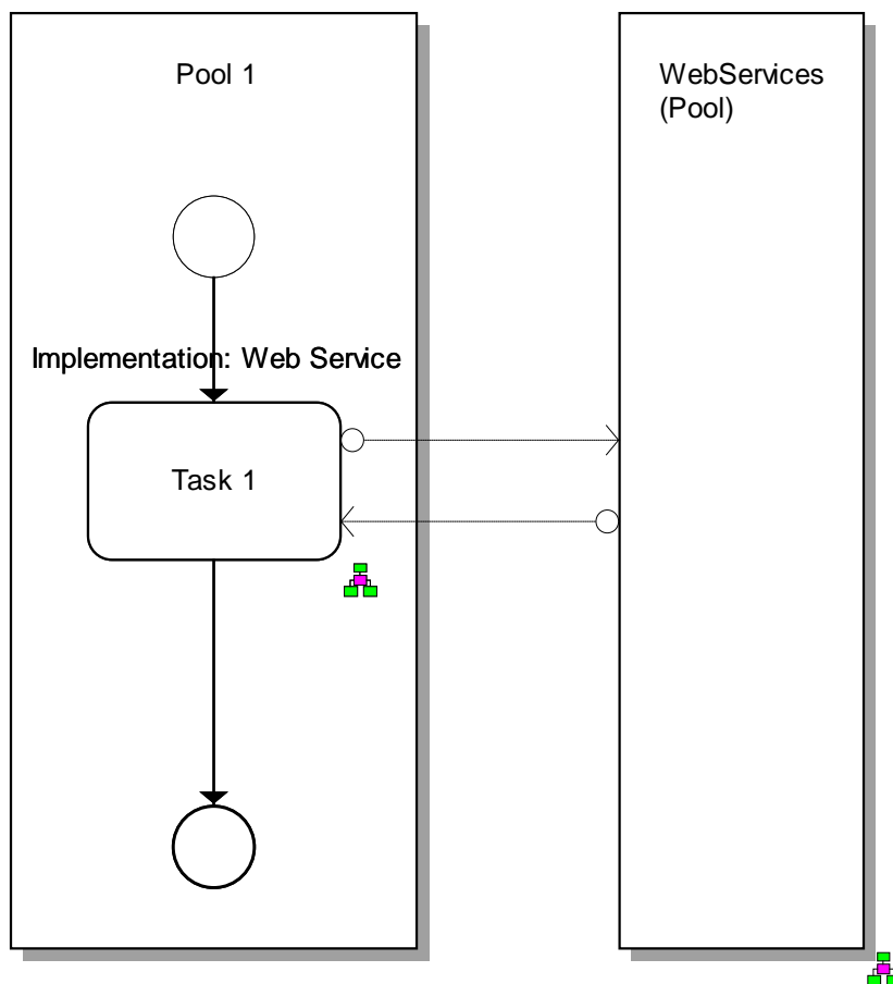
Figure 13: Task 1 has a Web Service Implementation; The Participant that provides the Web Service is WebServices (Pool) – the definition which operation is being executed is done inside the allocation diagram which is assigned behind Task1 (Figure 14)
