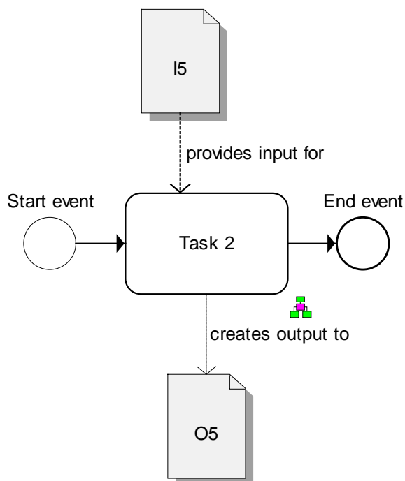
Figure 9: Simple Data Definition inside a BPMN Diagram – This diagram represents the same semantic than Figure 4, but can be modeled without an extra Allocation Diagram.
