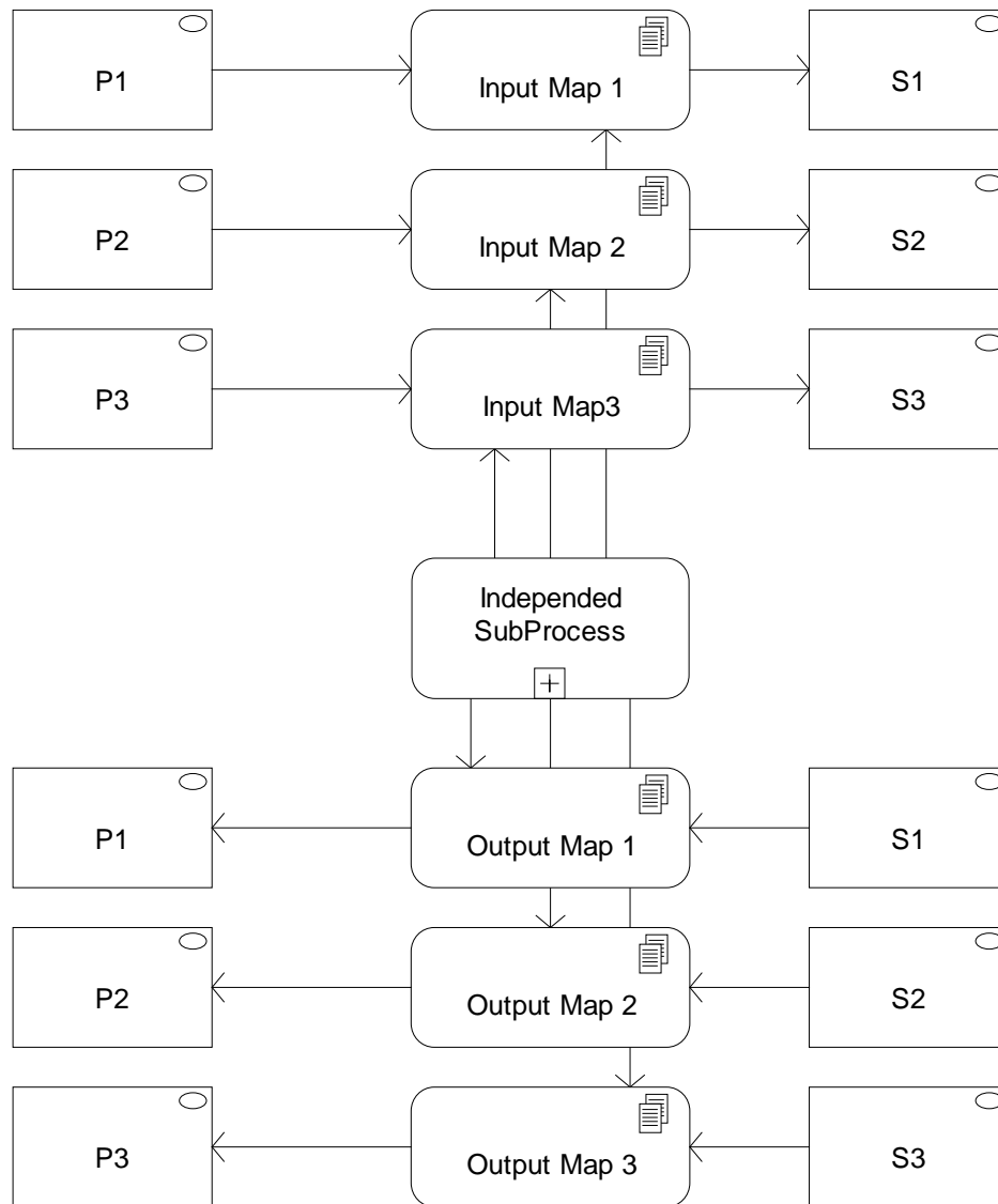
Figure 4: The Property Input/Output behavior of an independent sub process. P1, P2 and P3 are Occurrence copies of properties that are part of the parent process, S1-S3 are property objects that are part of the Independent Sub Process. The properties P1, P2 and P3 are transferred into the properties S1, S2 and S3 of the Sub Process. After the Sub Process has been completed the content S1 is copied into P1, S2 is copied into P2 and S3 is copied (mapped) to P3.
