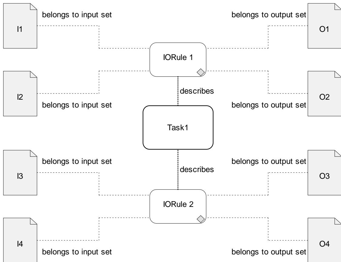
Figure 8: A Task with two input Sets ({I1, I2} {I3, I4}), two output sets ({O1, O2} {O3, O4}) and two corresponding IORules (IORule 1, IORule 2). Semantic: Task1 can be instantiated if I1 AND I2 are available OR if I3 AND I4 are available. If the Task is instantiated with I1 AND I2 it will produce O1 AND O2, if the Task was instantiated with I3 AND I4 it will produce O3 AND O4.
