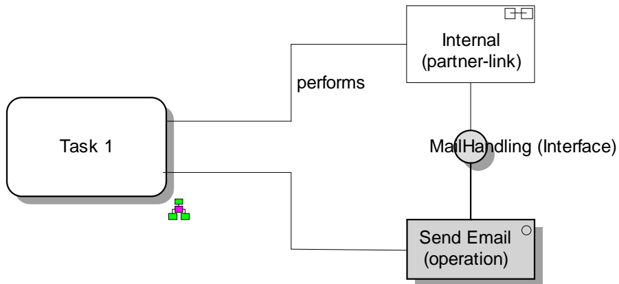
Figure 14: The allocation Diagram behind Task1 – Task 1 executes the Operation SendEMail from the Interface MailHandling on the PartnerLink internal
