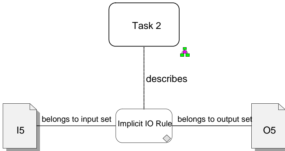
Figure 10: Exact modeling of Figure 11 inside a BPMN Allocation Diagram – this diagram represents the same semantic as Figure 12
