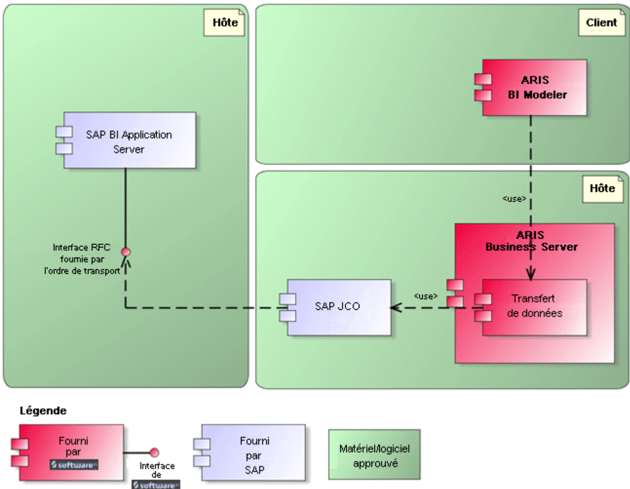
Figure 4: BI Modeling
