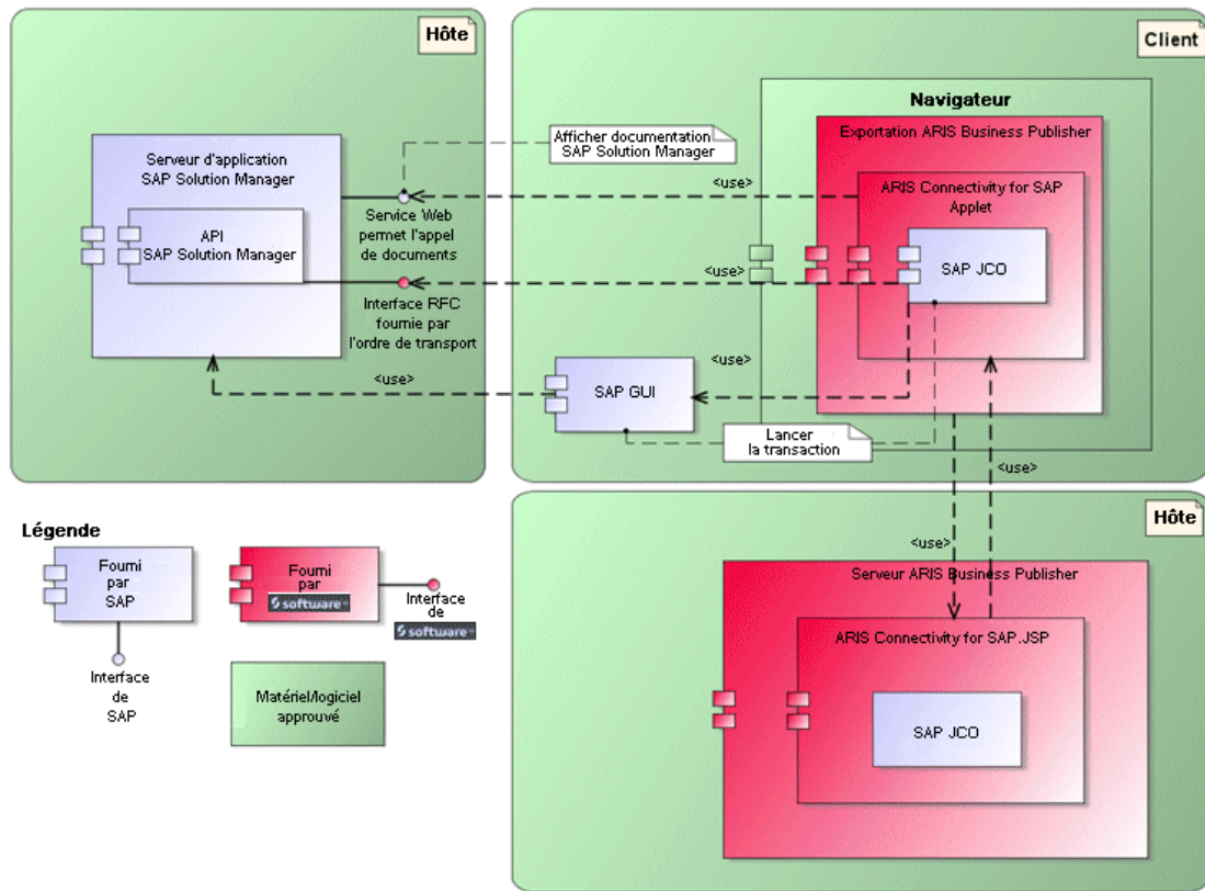
Figure 3: ARIS Publisher
