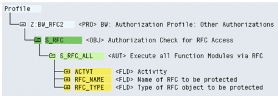
Figure 11: Profil SAP®
