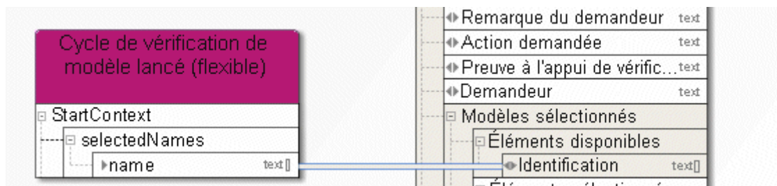
Figure 6: Listes
