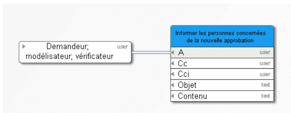
Figure 7: Exemple 1 – Information
