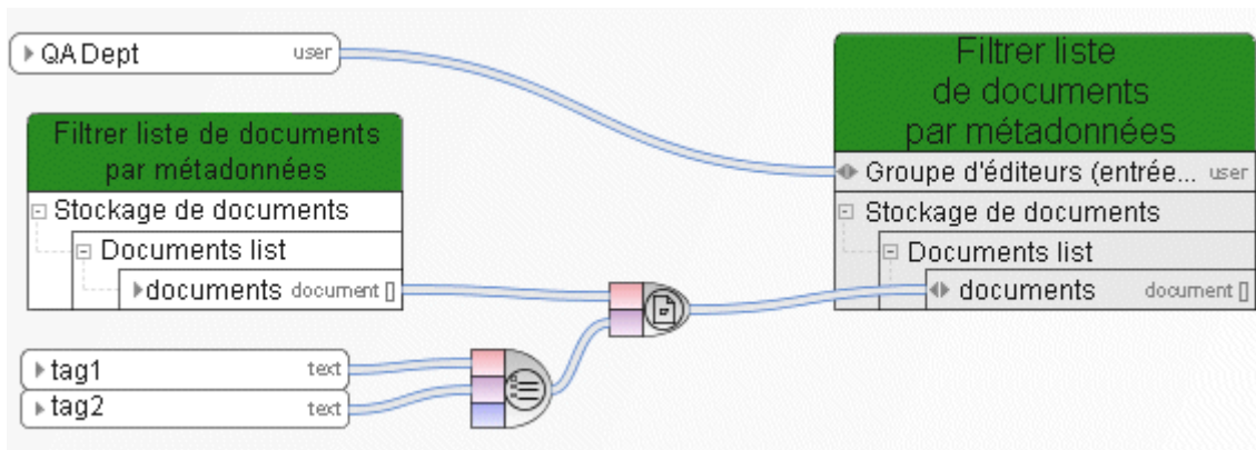
Figure 109: Filtrer documents
