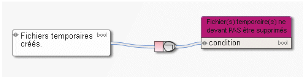
Figure 98: NOT
