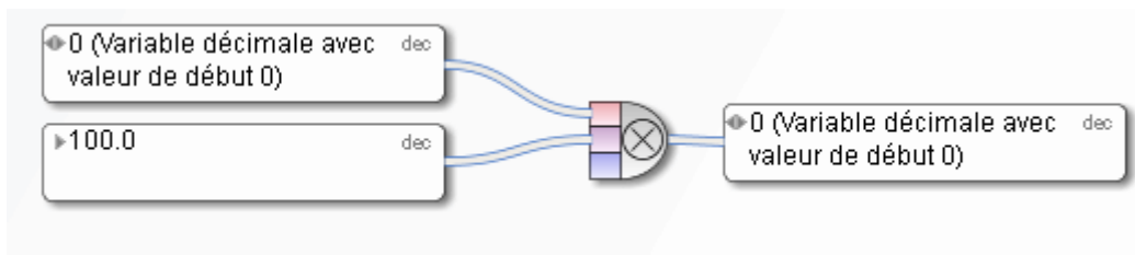
Figure 88: Multiplier
