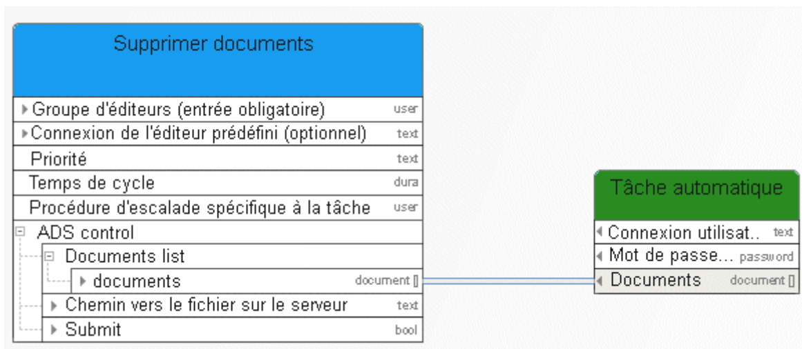
Figure 49: Supprimer document
