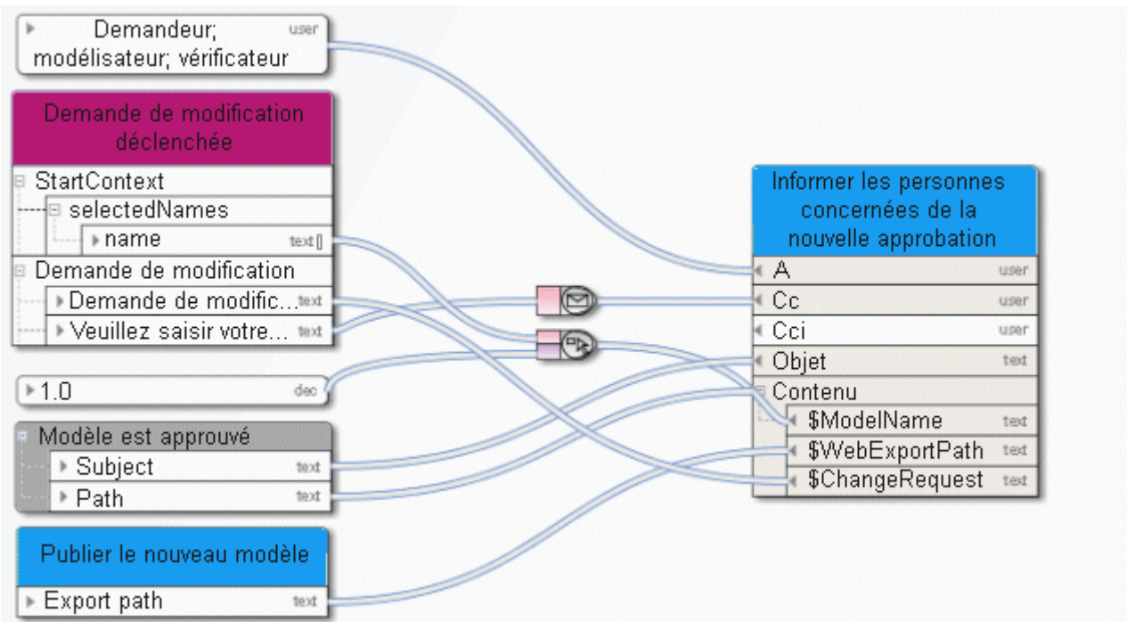
Figure 8: Exemple 2 – Information
