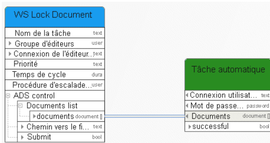
Figure 51: Verrouiller documents
