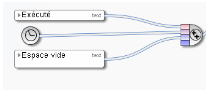
Figure 112: Fournir horodatage
