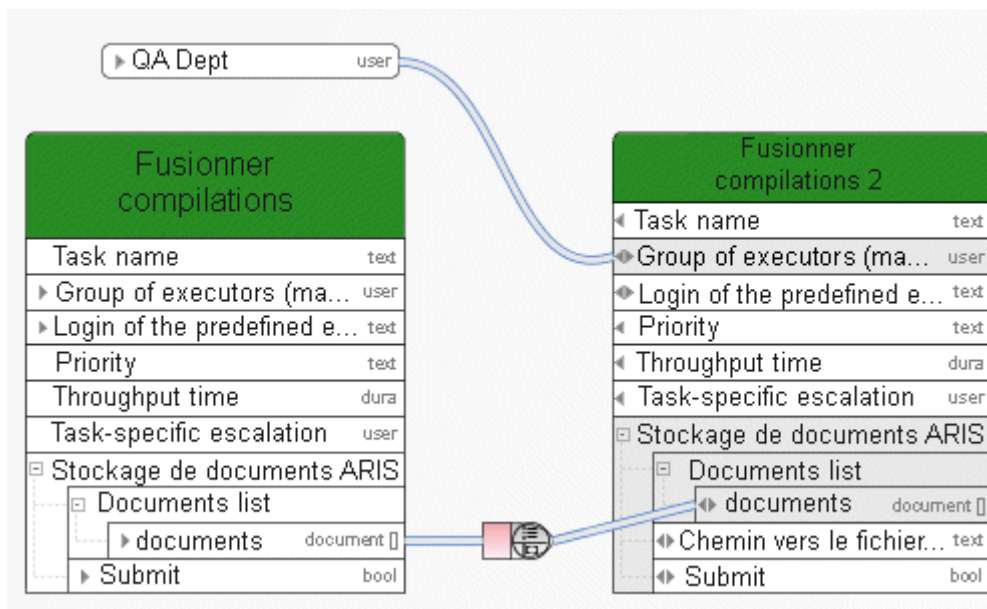
Figure 105: Valider compilation
