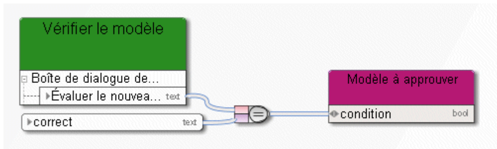
Figure 121: Constantes
