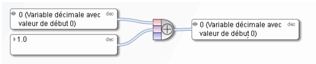
Figure 85: Additionner
