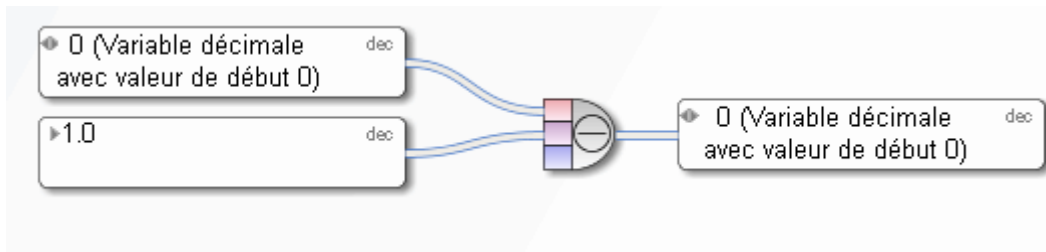
Figure 86: Soustraire
