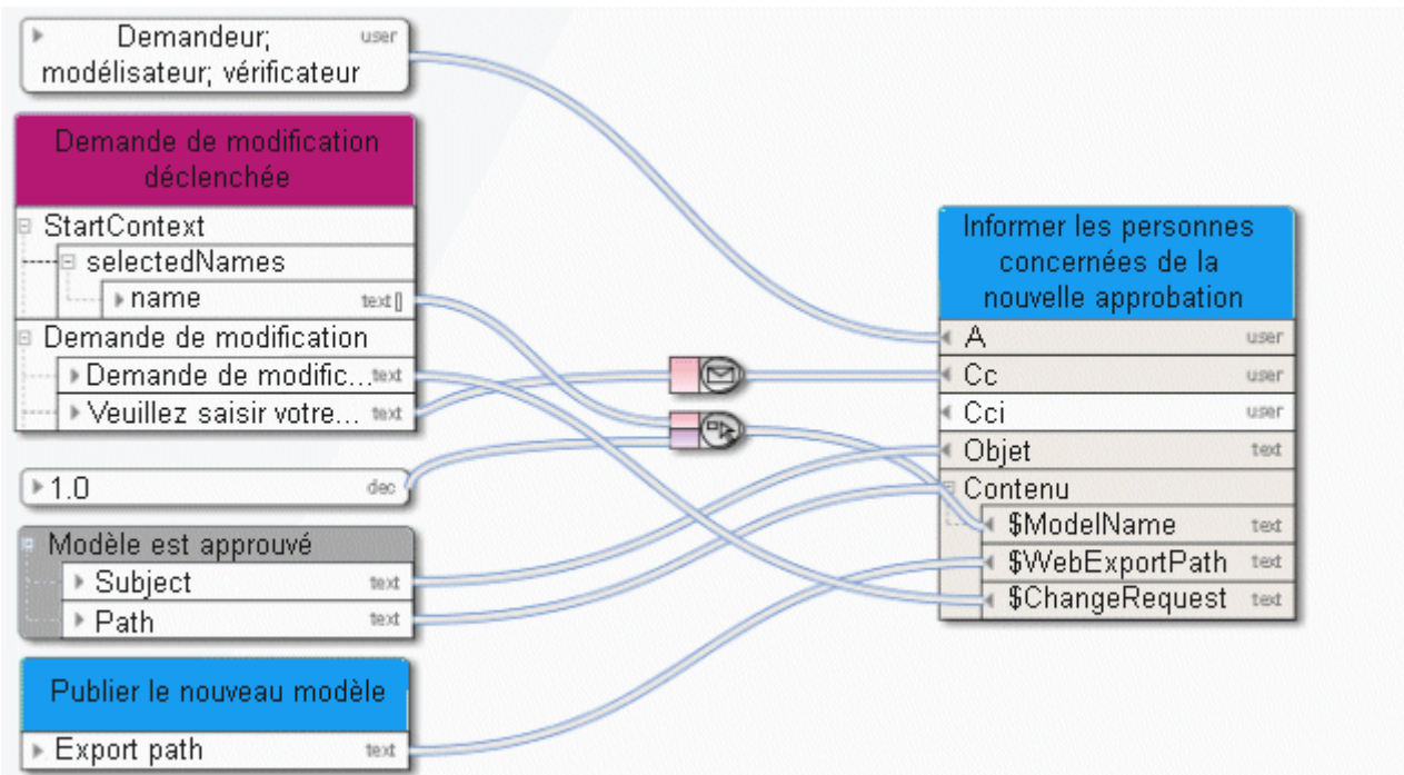
Figure 8: Exemple 2 – Information
