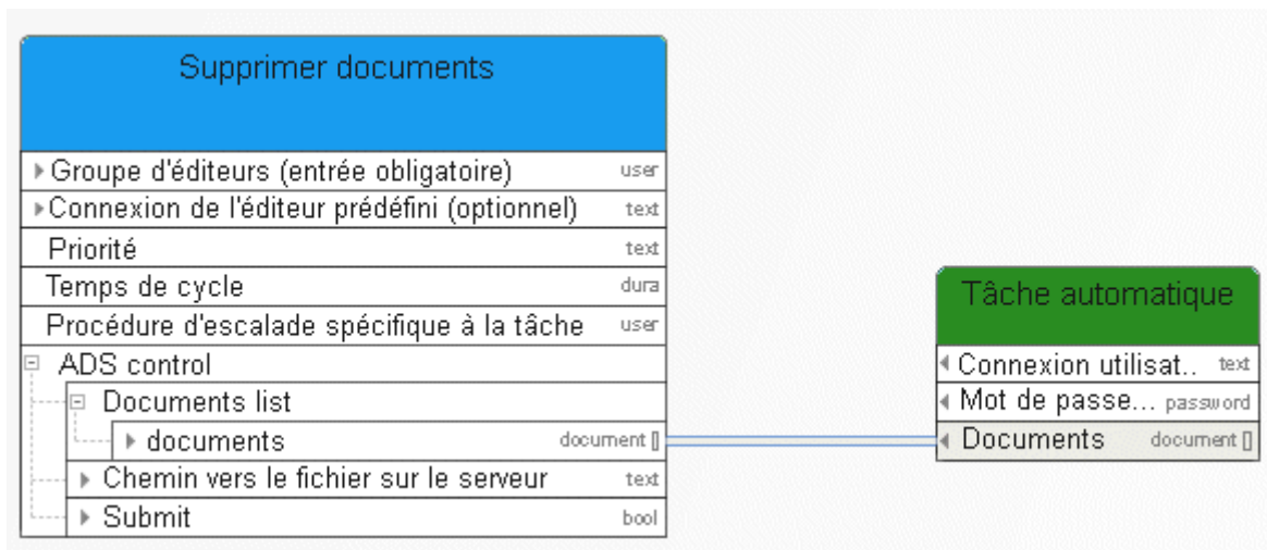
Figure 48: Supprimer document
