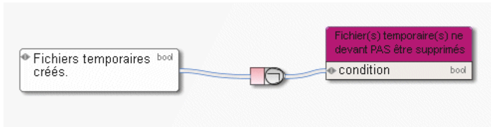
Figure 97: NOT
