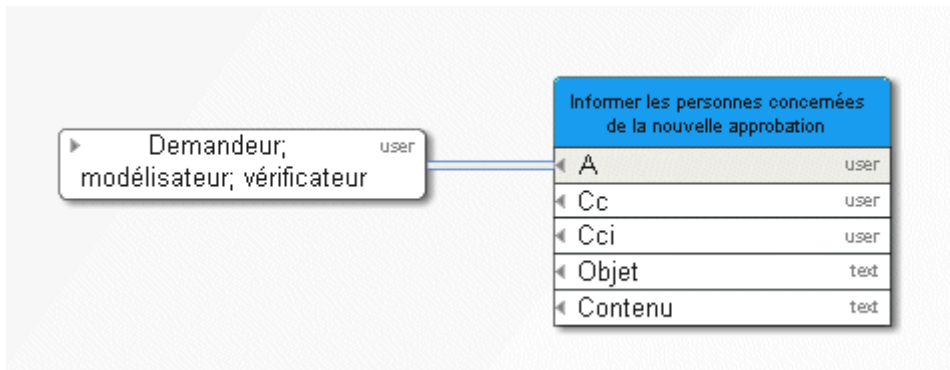
Figure 7: Exemple 1 – Information
