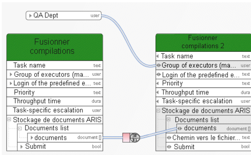
Figure 104: Valider compilation
