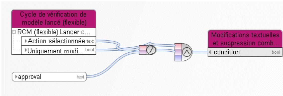
Figure 95: ET
