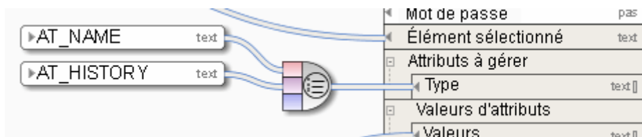
Figure 100: Créer compilation
