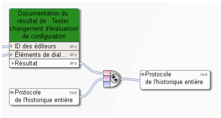
Figure 116: Lier
