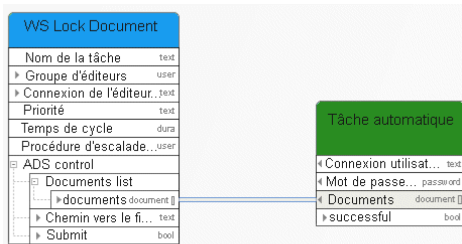
Figure 50: Verrouiller documents
