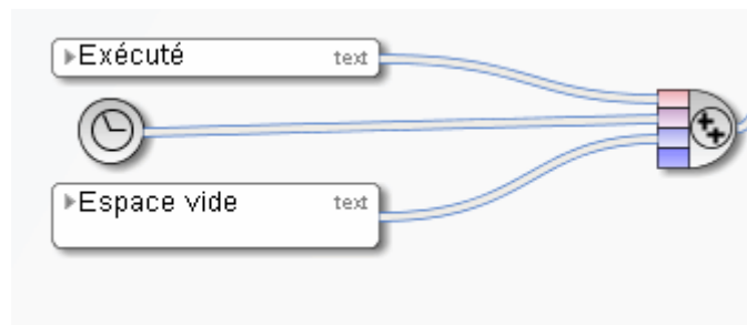
Figure 111: Fournir horodatage
