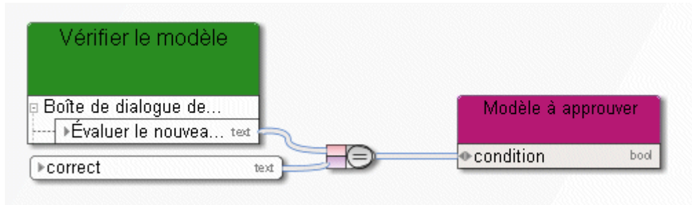
Figure 120: Constantes
