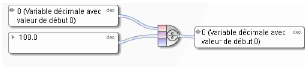
Figure 88: Diviser
