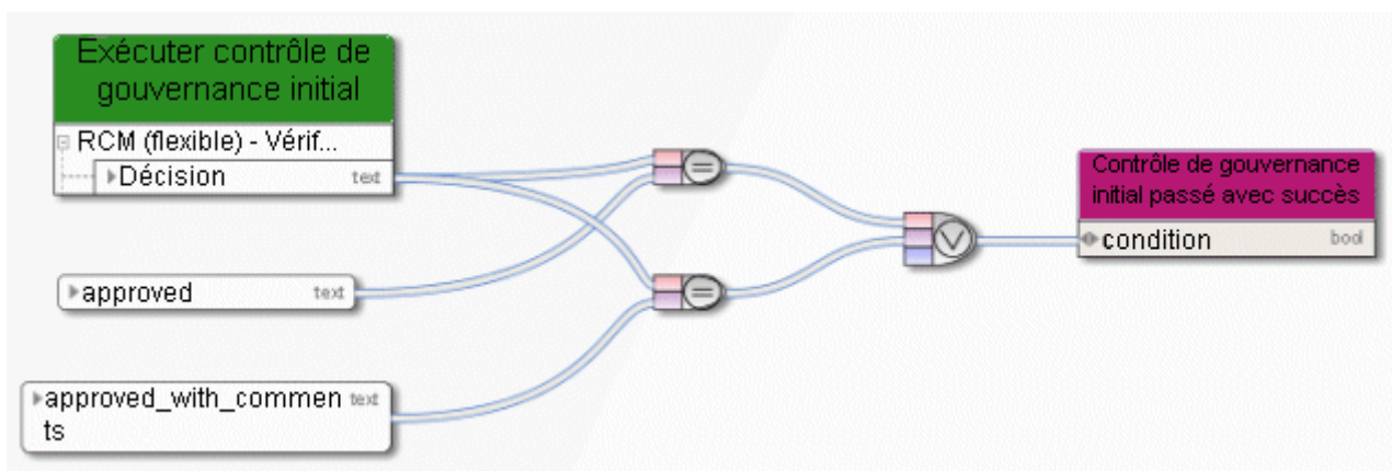
Figure 96: OU
