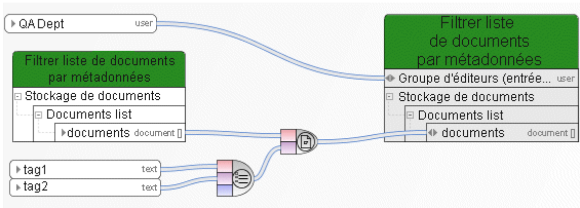
Figure 108: Filtrer documents
