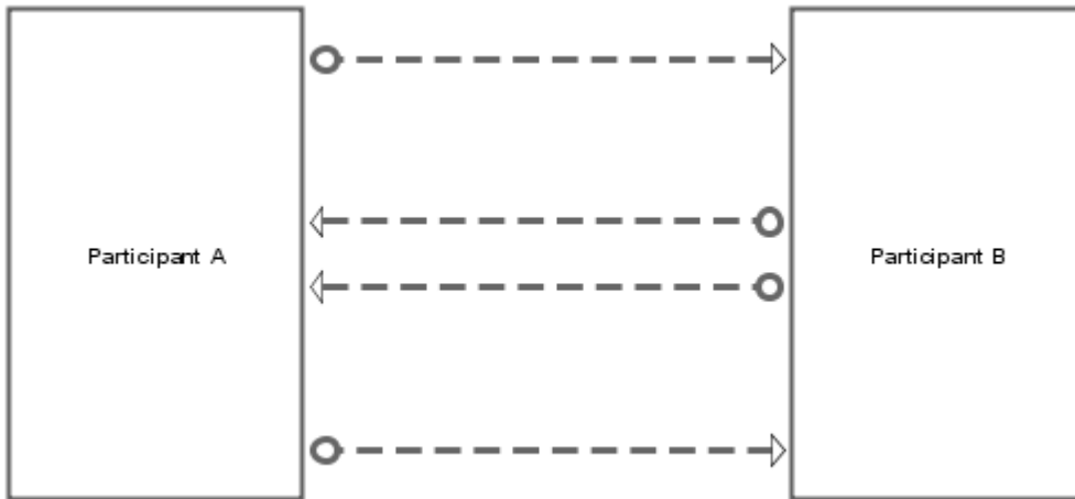
Illustration 176: Message flow between Participants in a BPMN conversation diagram (BPMN 2.0)
