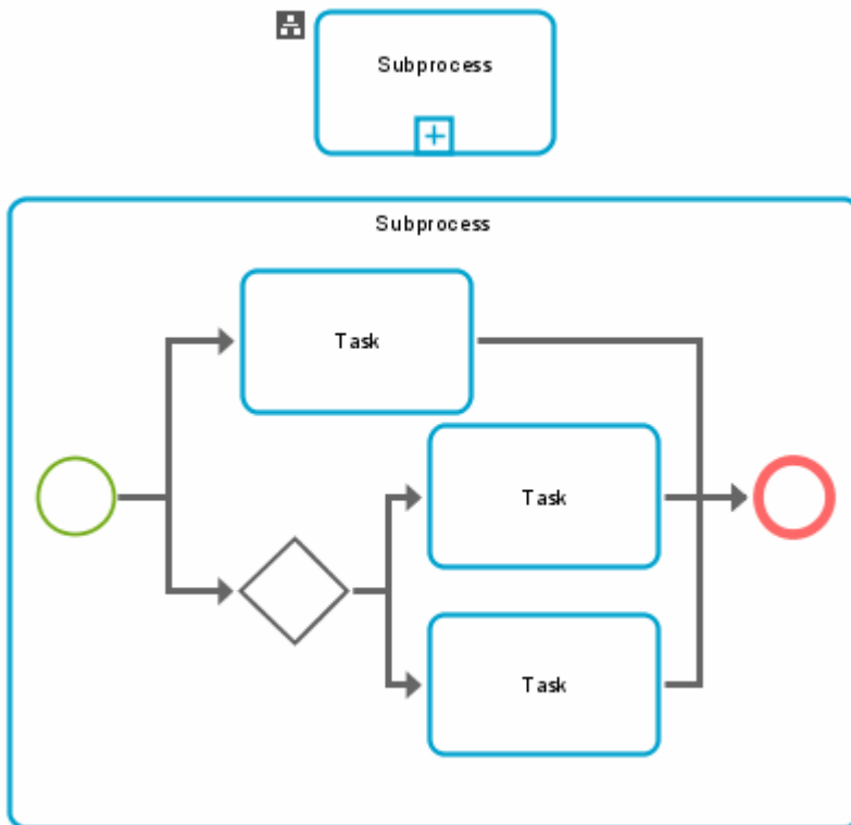
Illustration 163: Symbols of a standard subprocess
