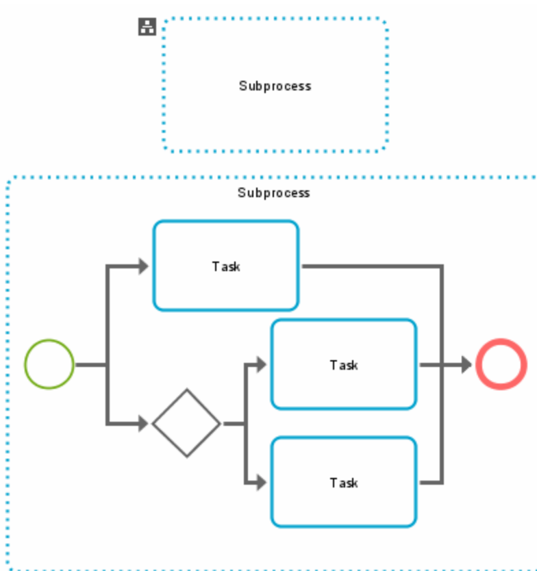
Figure 162: Symbols of an event subprocess
