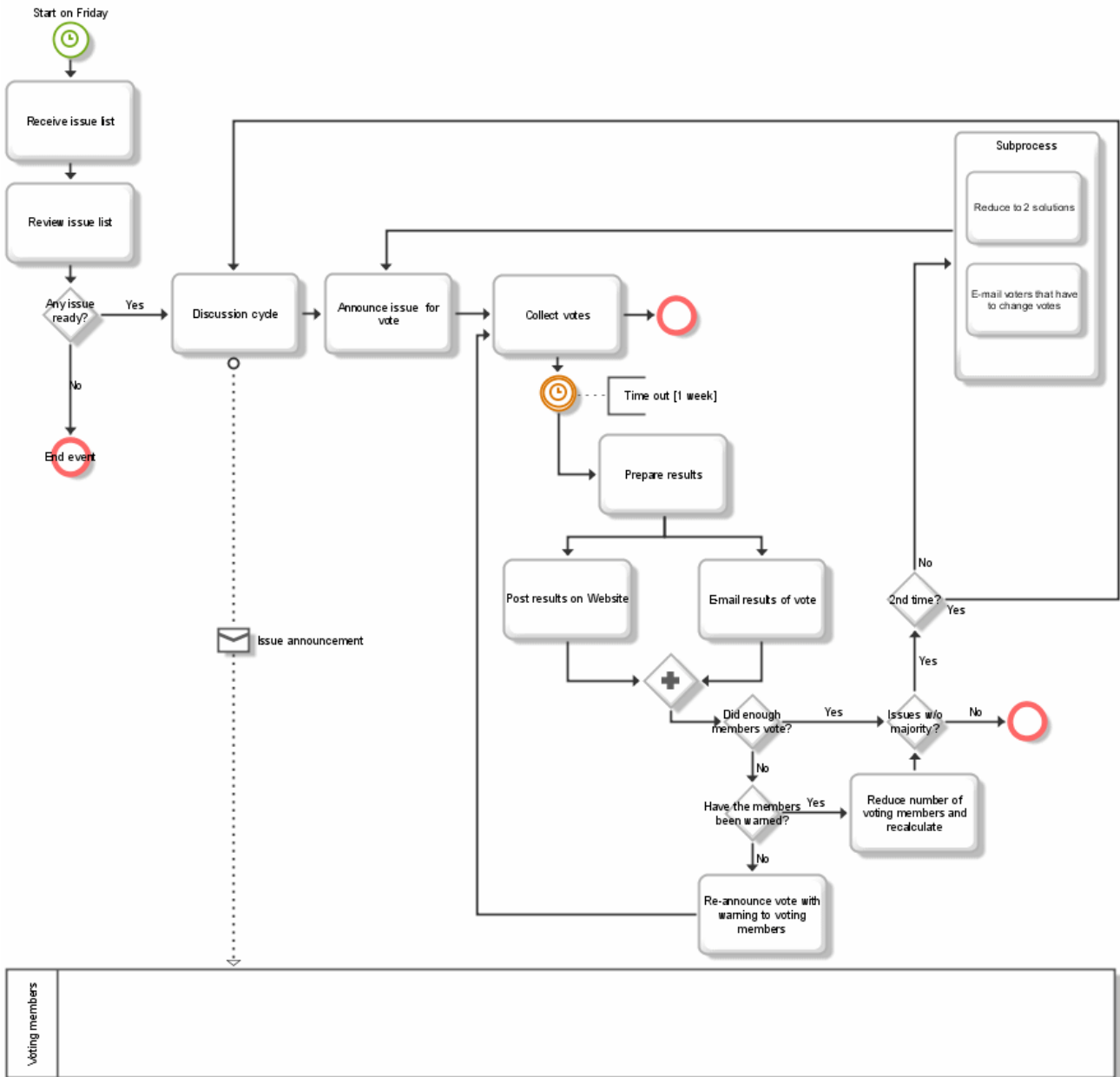
Abbildung 214: E-Mail Voting Process
