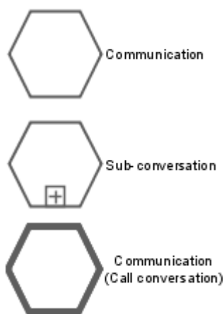
Abbildung 234: Symbols of Conversation nodes
