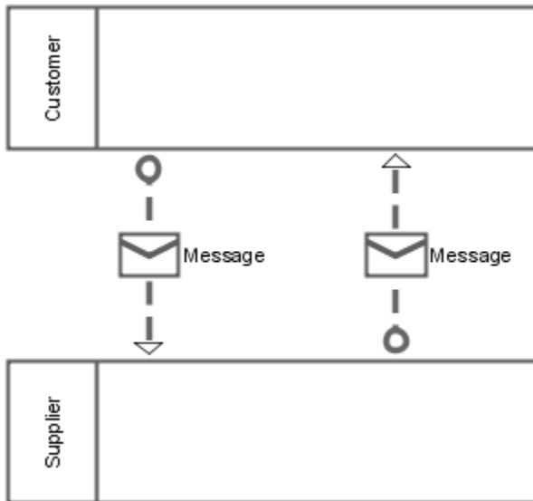
Abbildung 219: Message flow between participants/pools
