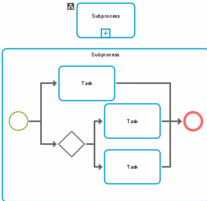
Abbildung 223: Symbols of a standard subprocess
