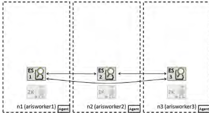
Figure 34: The elasticsearch cluster in our example scenario
