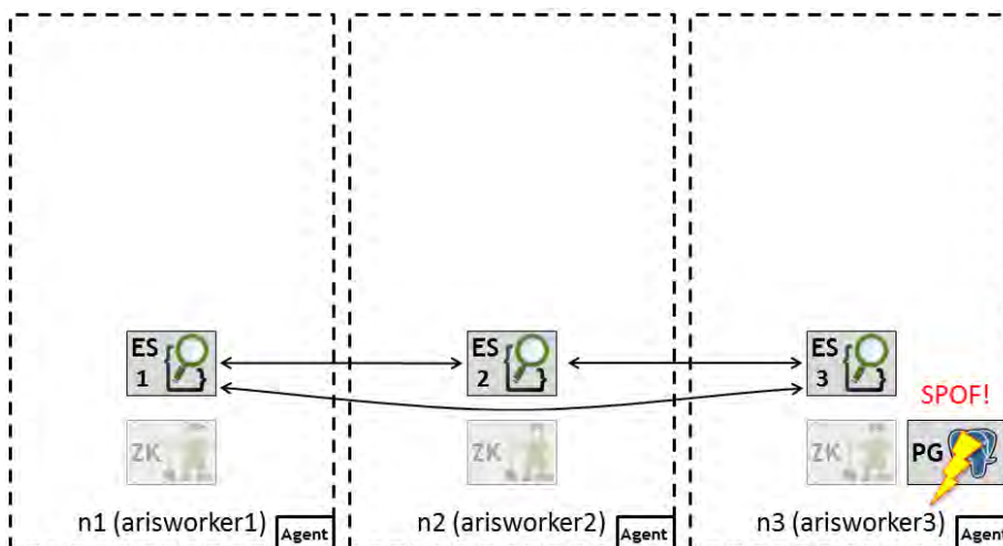
Figure 37: Our distributed example scenario when using the PostgreSQL runnable instead (i.e., no high availability, strictly exercise only)
