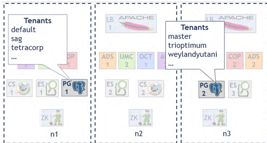
Figure 35: A possible distribution of tenants across multiple PostgreSQL instances
