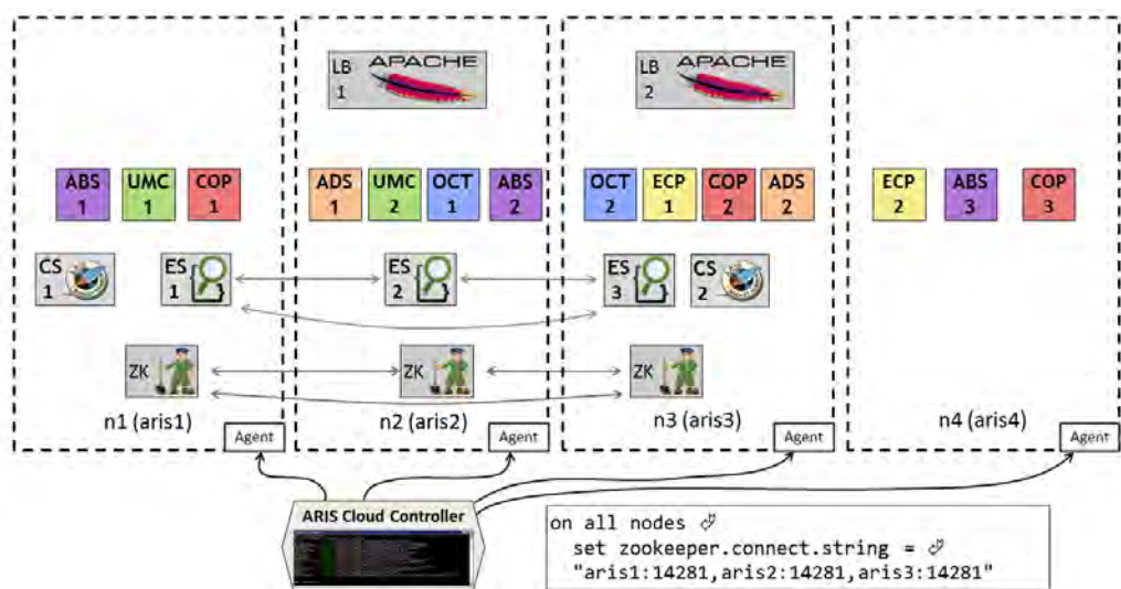
Figure 26: Automatic setting of the zookeeper.connect.string by the ACC
