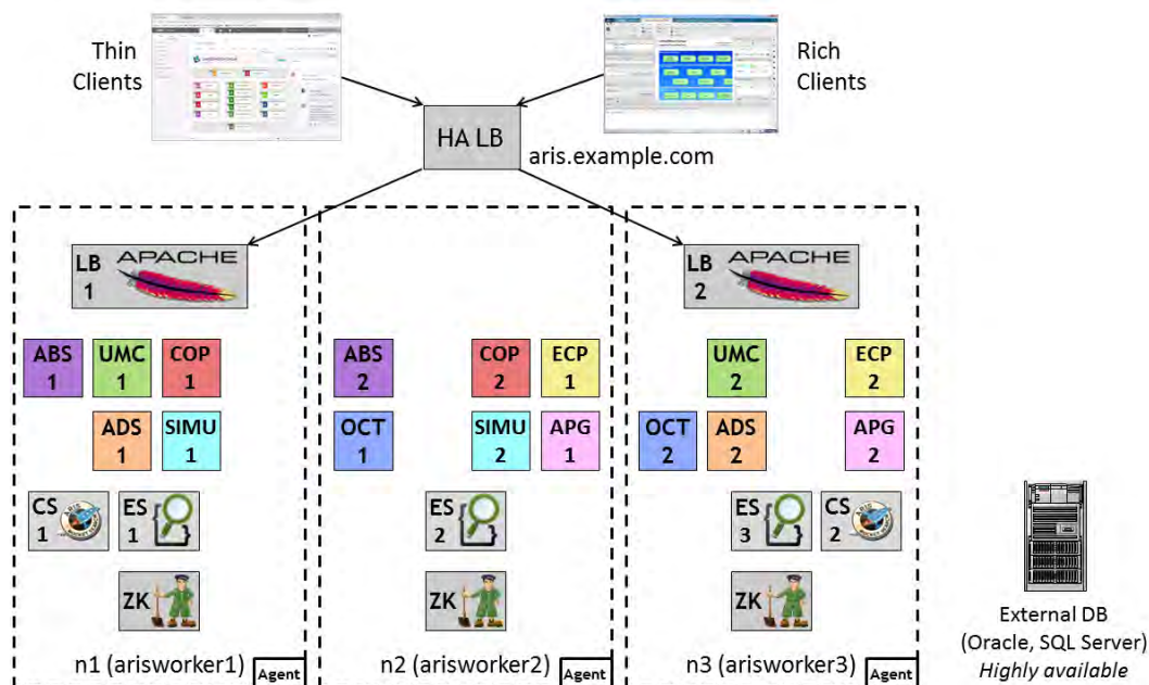
Figure 57: Our distributed example scenario
