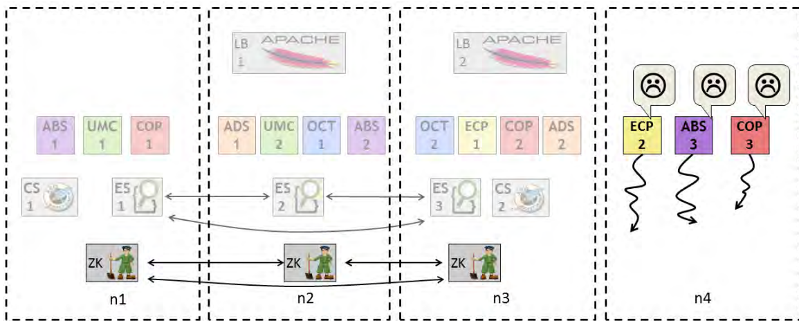
Figure 24: A node without a local Zookeeper instance
