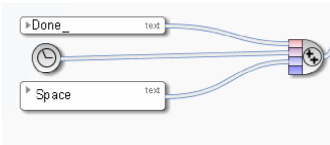
Figure 120: Get timestamp
