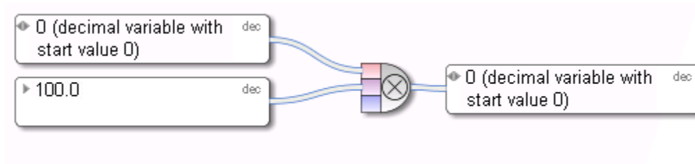
Figure 96: Multiply
