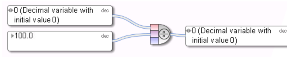
Figure 97: Divide
