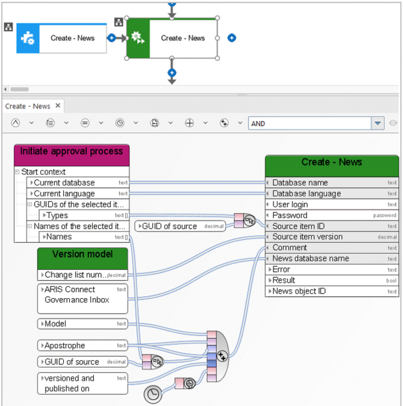
Figure 18: Create - News
