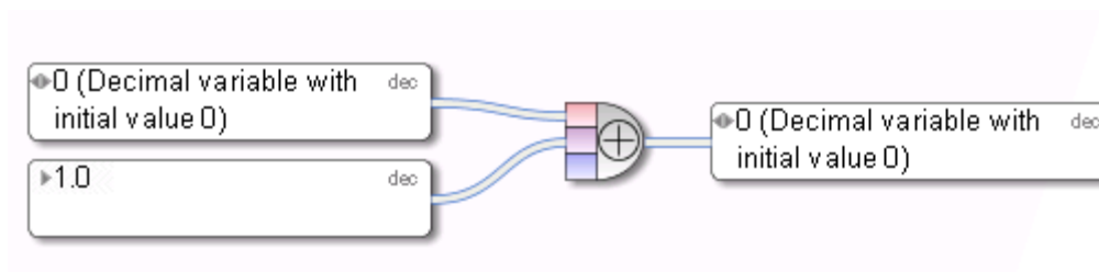
Figure 94: Add
