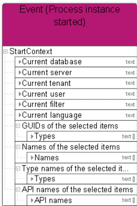
Figure 1: Start context
