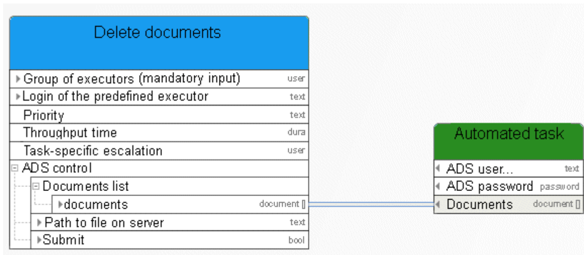
Figure 54: Delete document
