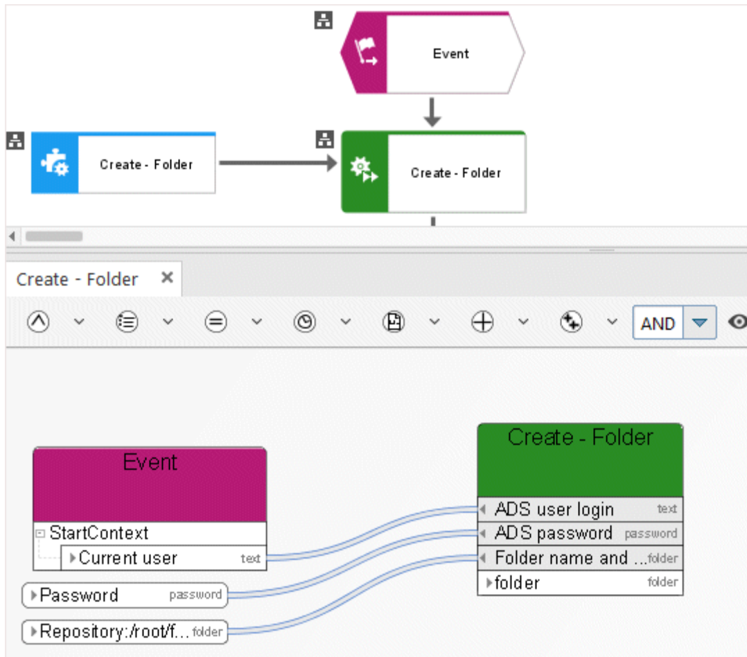
Figure 53: Create folder
