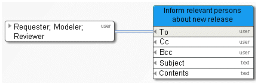
Figure 7: Example 1 – Notification
