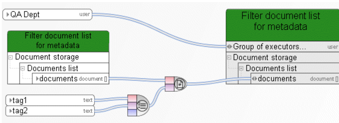
Figure 117: Filter documents
