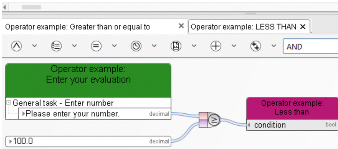
Figure 102: Less than
