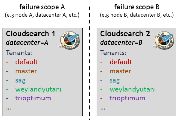
FIGURE 41: TWO CLOUDSEARCH INSTANCES ASSIGNED TO TWO DIFFERENT DATA CENTERS
