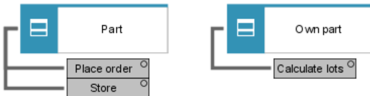
Figure 156: Assignment of operations to classes
