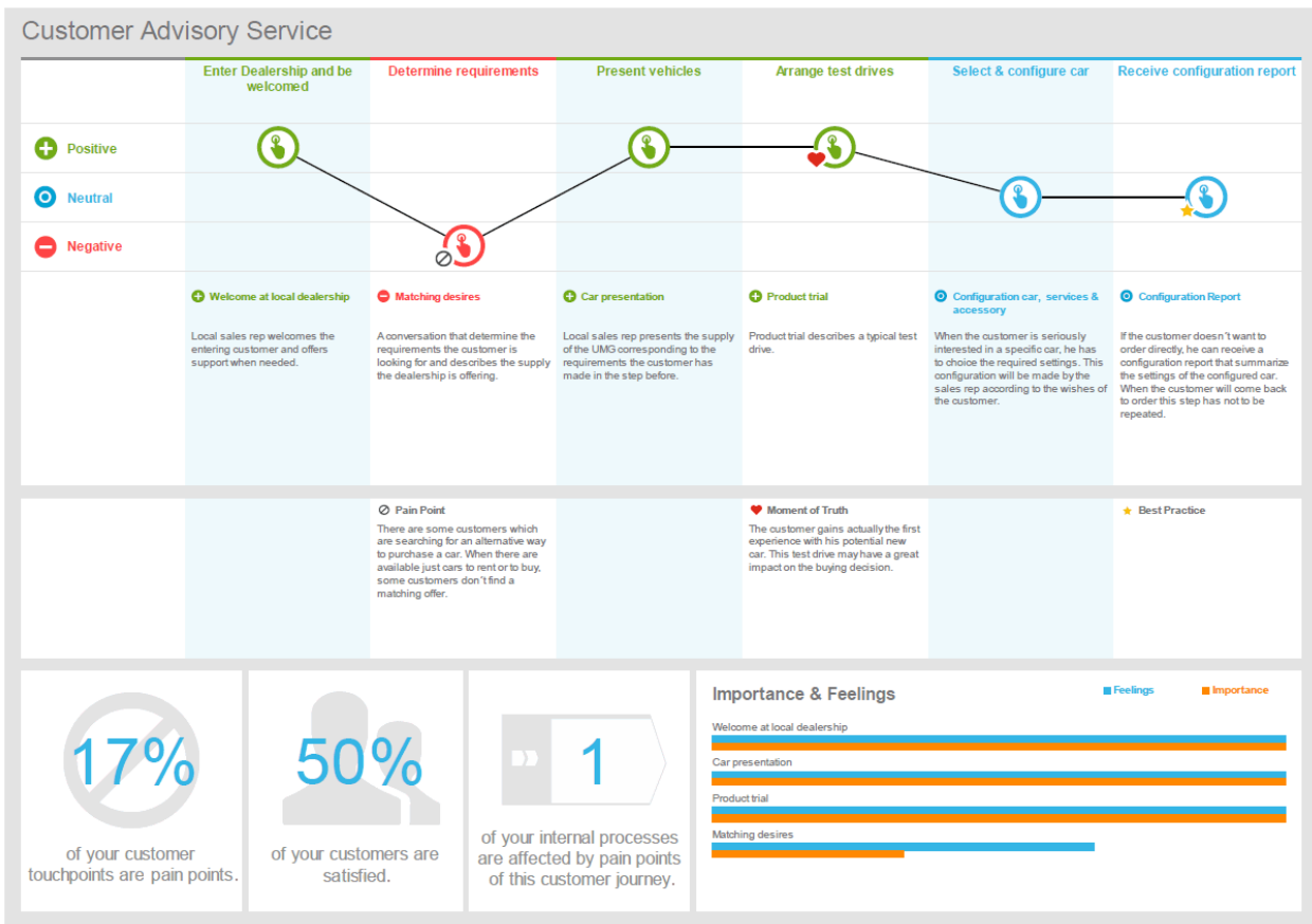
Figure 243: CXM infographic
