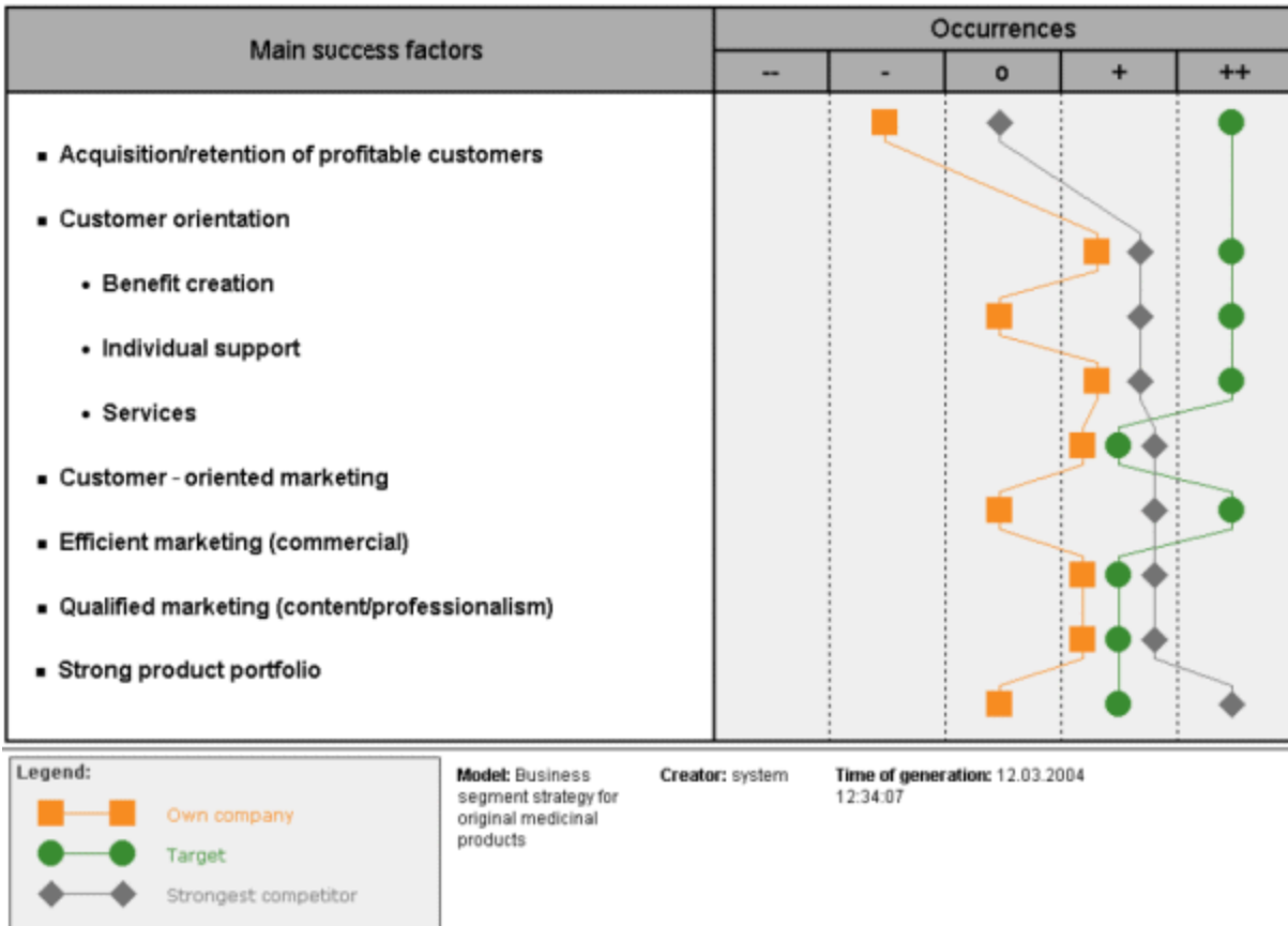
Figure 129: Report
