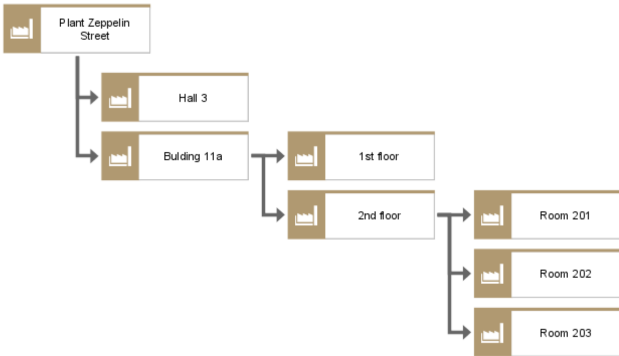
Figure 79: Location hierarchies
