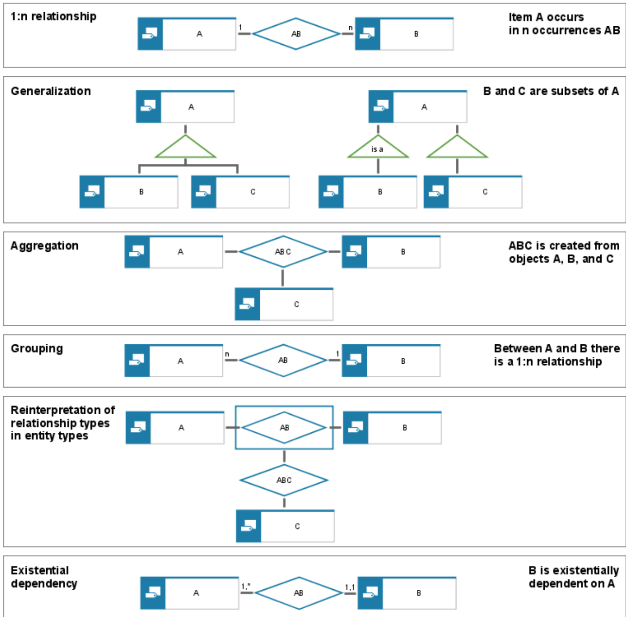
Figure 52: eERM: Terms and forms of representation
