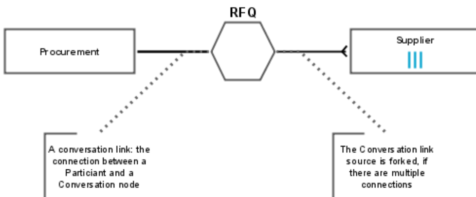
図 173: Conversation link with Participant multiplicity
