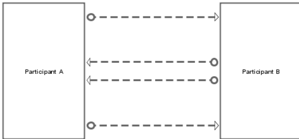
図 176: Message flow between Participants in a BPMN conversation diagram (BPMN 2.0)
