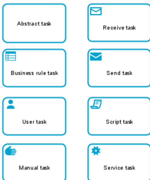
Figure 160: Task symbols
