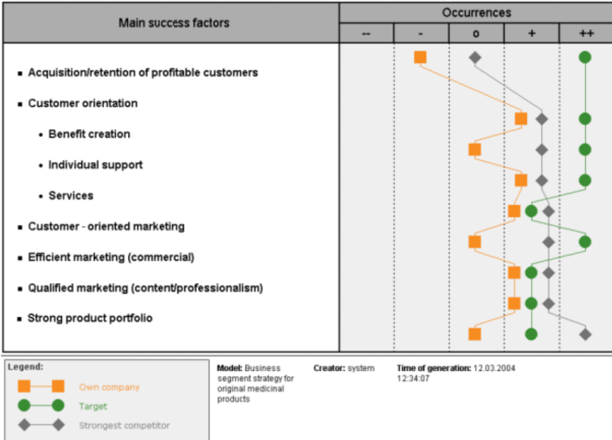
Figure 97: Report
