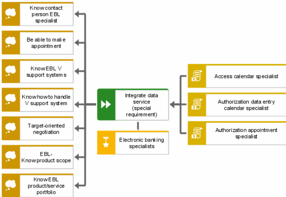
Figure 93: Role diagram
