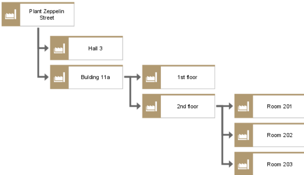
Figure 61: Location hierarchies
