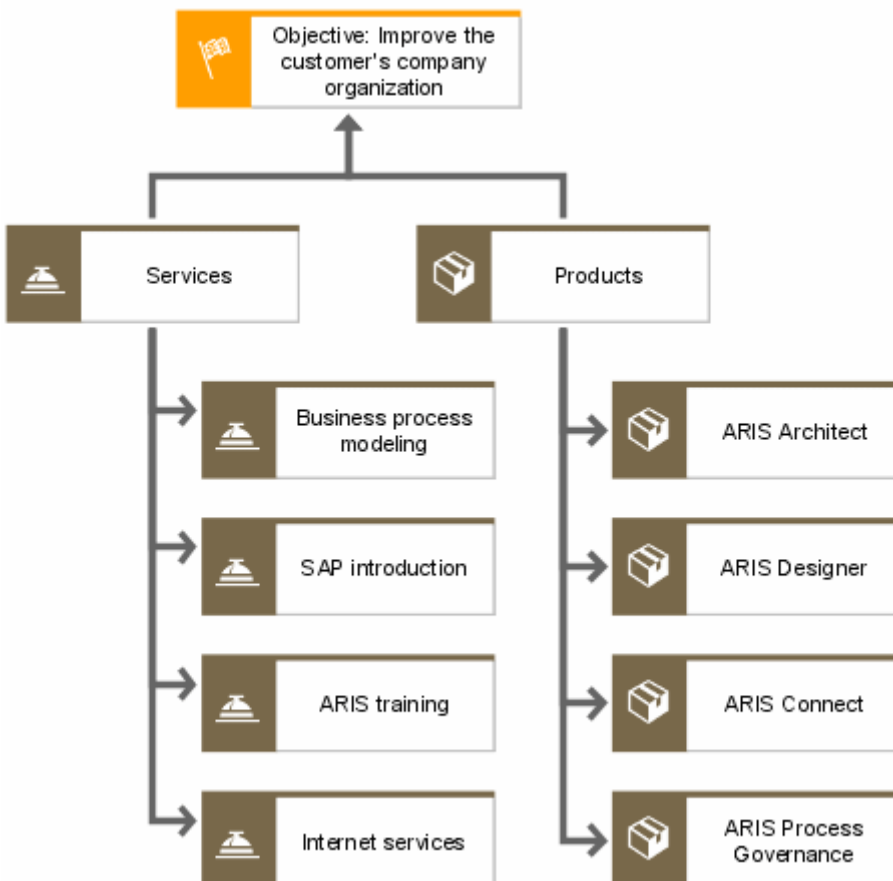
Figure 111: Product/Service tree
