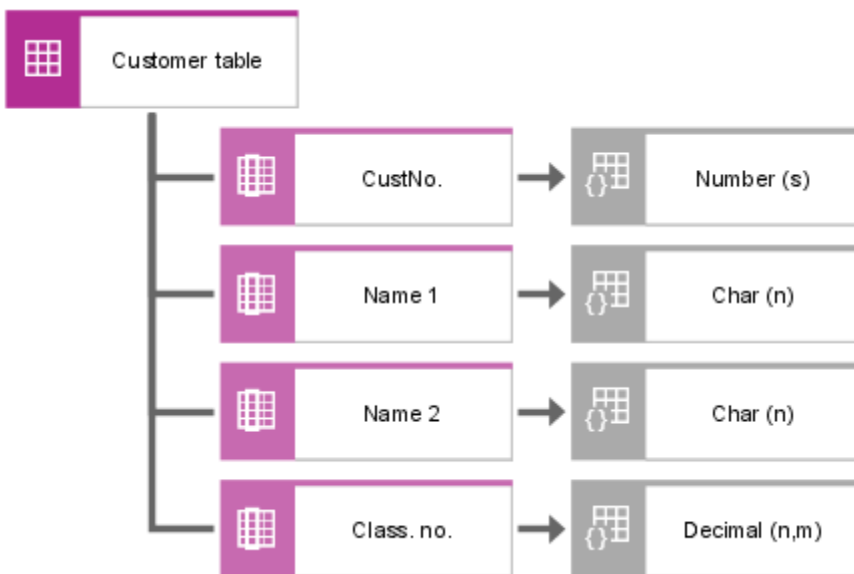
Figure 51: Field allocations
