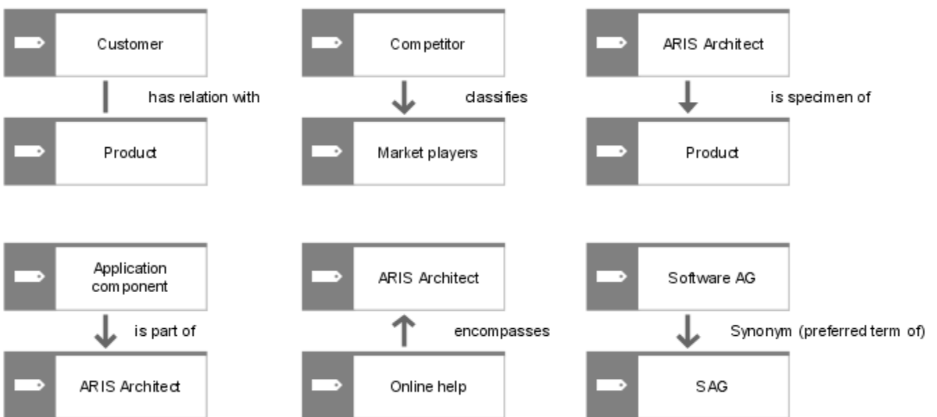
Figure 43: Technical terms (2)
