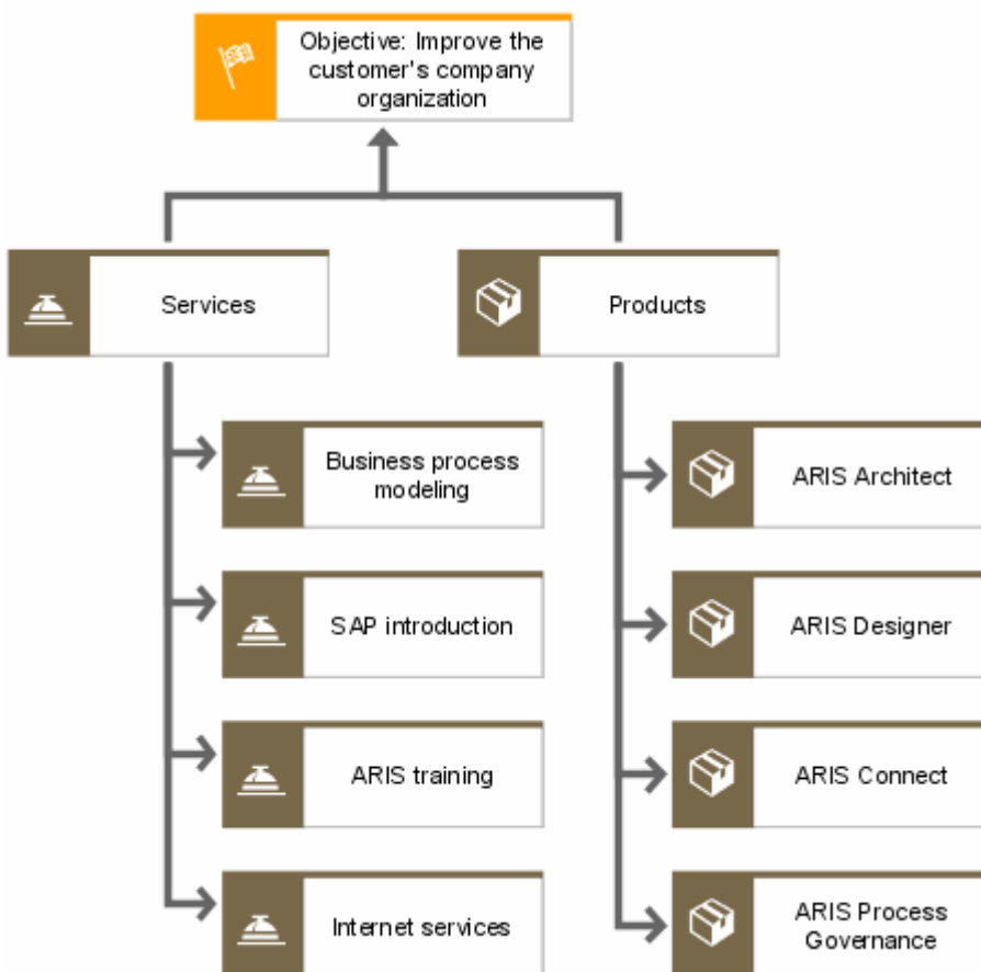
Figure 111: Product/Service tree
