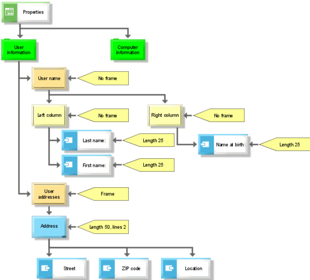
Figure 102: Example of a screen diagram
