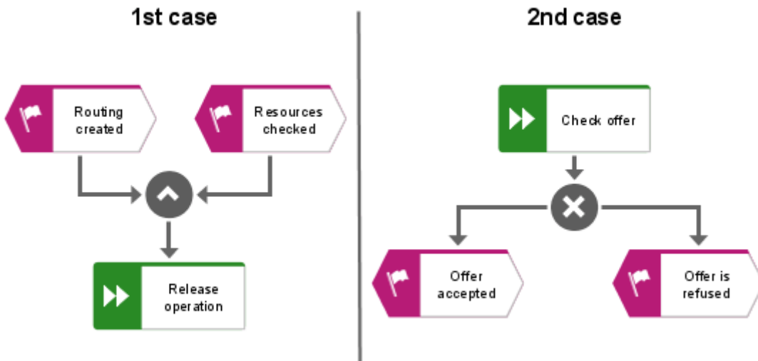
Figure 70: Examples of rules
