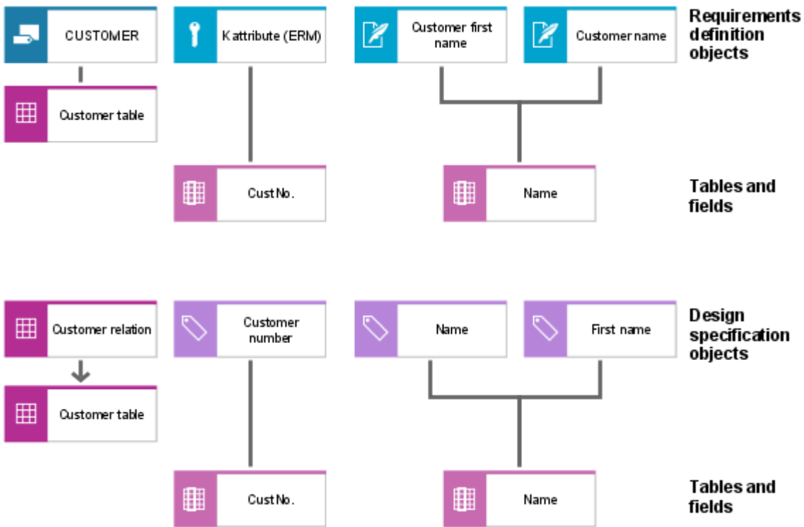
Figure 52: Allocation of requirements definition and design specification objects
