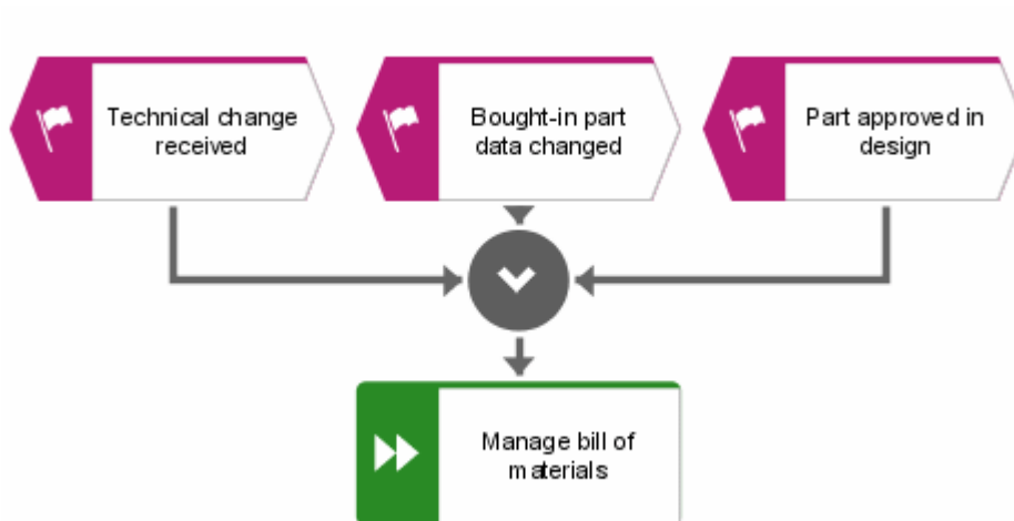
Figure 73: OR operator for triggering events
