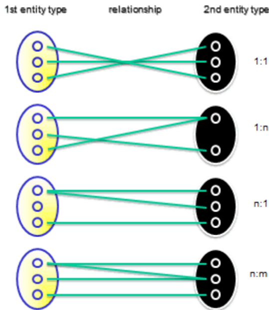
Figure 25: Cardinalities of relationships between two entity types
