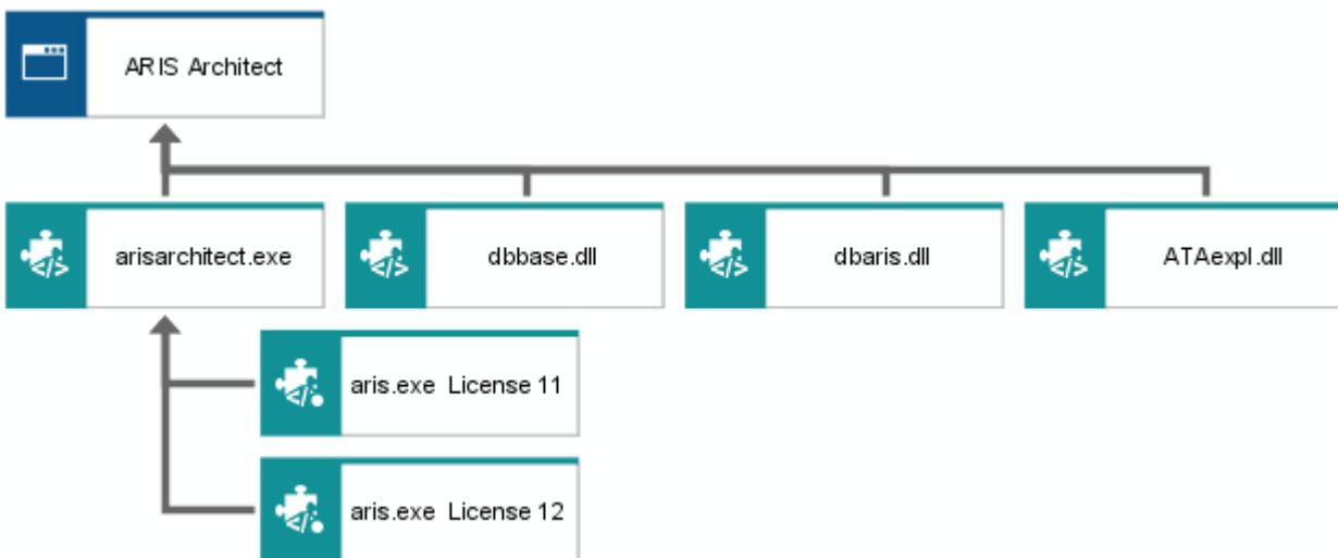
Figure 21: Assignment of application system types, program module types, and program modules
