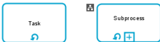
Abbildung 167: Symbols of Standard loop activities
