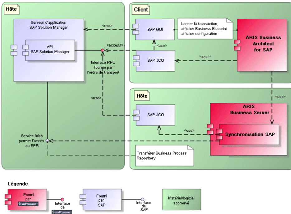
Figure 1: Synchronisation SAP®, Lancer la transaction, Afficher Blueprint
