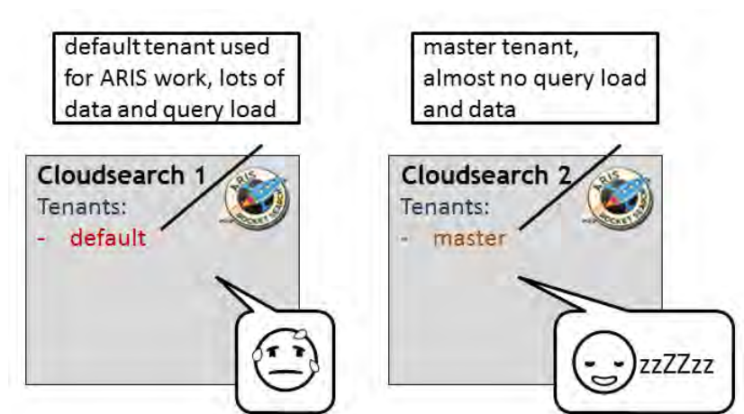
Figure 43: One active tenant and two Cloudsearch instances
