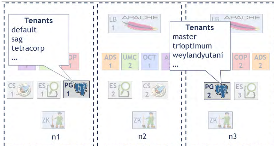
Figure 35: A possible distribution of tenants across multiple PostgreSQL instances
