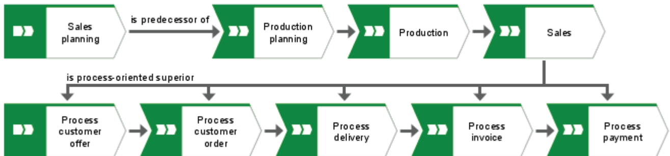
Figure 86: Value-added chain
