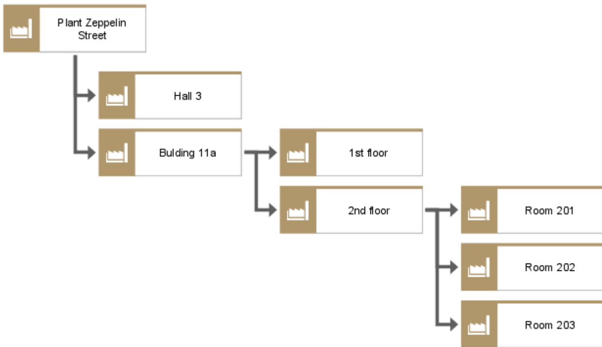
Figure 61: Location hierarchies
