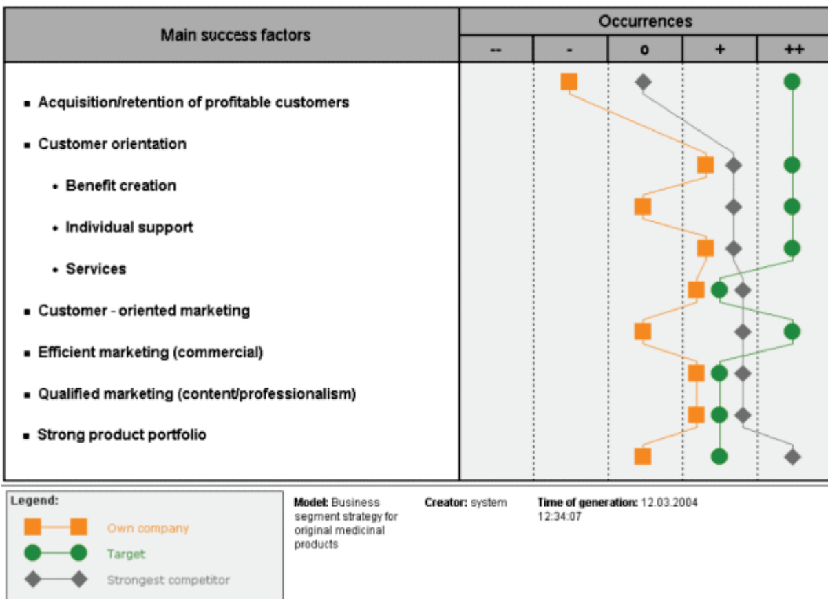
Figure 97: Report
