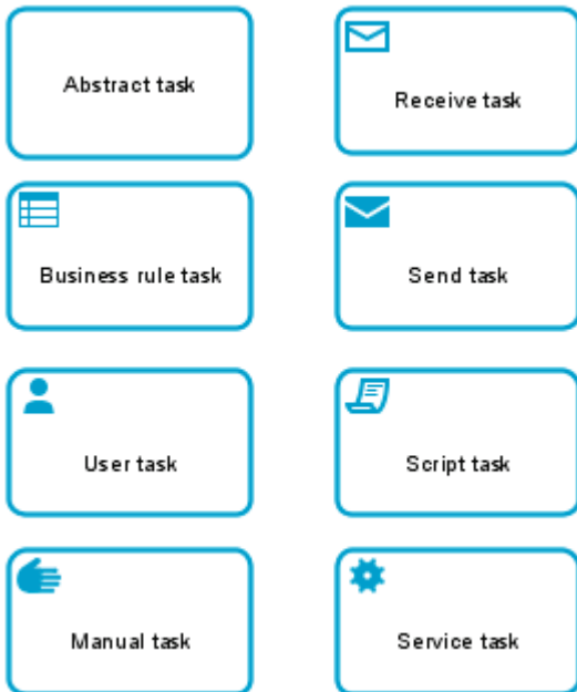
Figure 160: Task symbols
