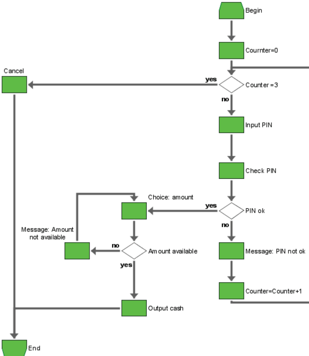
Figure 101: Example of a program flow chart (PF)
