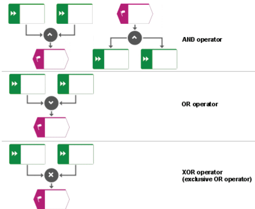
Figure 71: Logic operators (rules)
