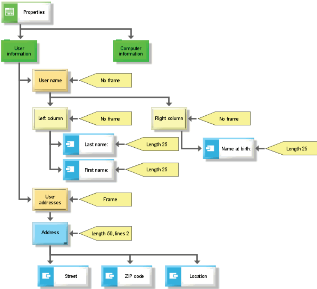
Figure 102: Example of a screen diagram
