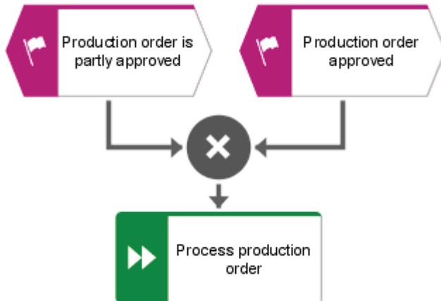
Figure 74: XOR operator for triggering events
