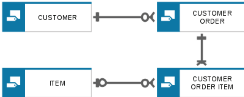
Figure 46: Data model in IE notation
