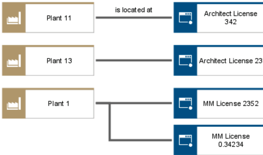
Figure 109: Location assignments
