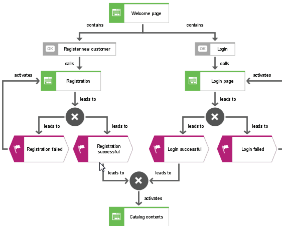
Figure 95: Example of screen navigation with events
