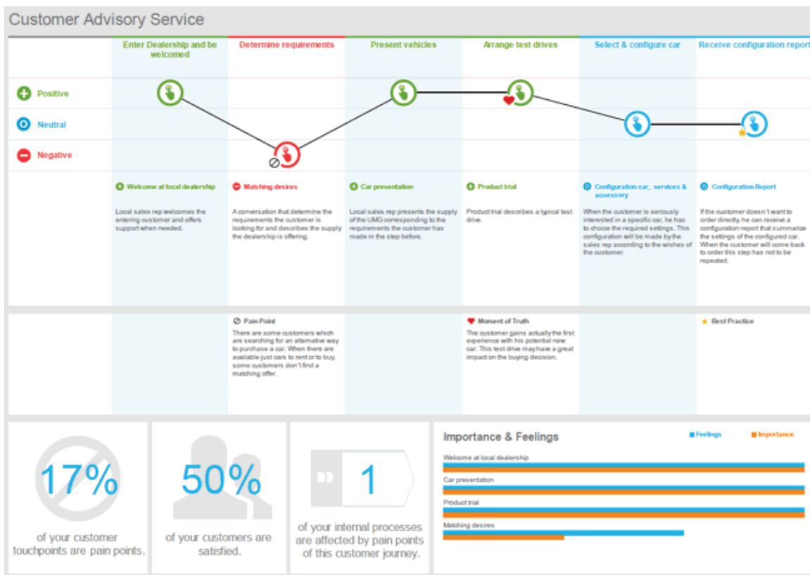
Figure 181: CXM infographic
