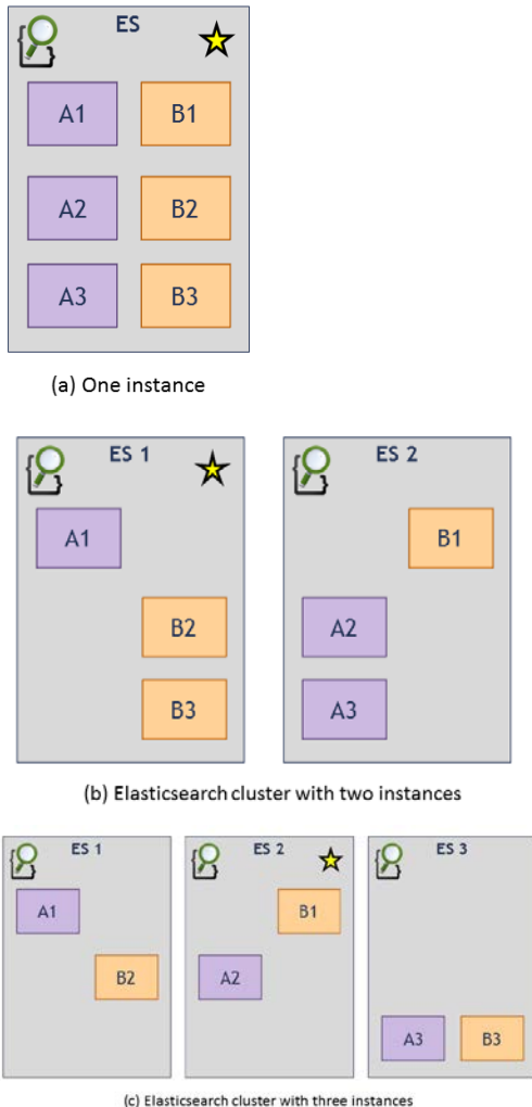
FIGURE 32: DISTRIBUTION OF THE SHARDS OF AN ELASTICSEARCH INDEX ACROSS A CLUSTER
