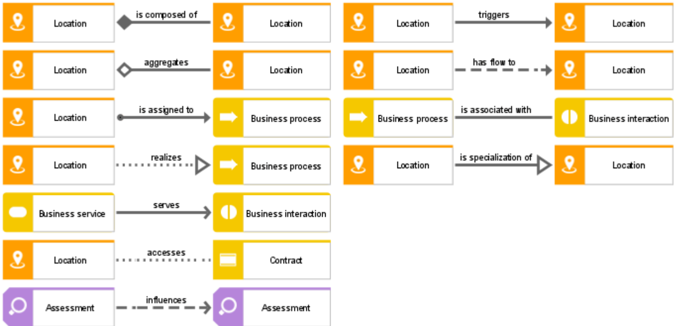
Figure 11: ArchiMate® 3.0: relationships
