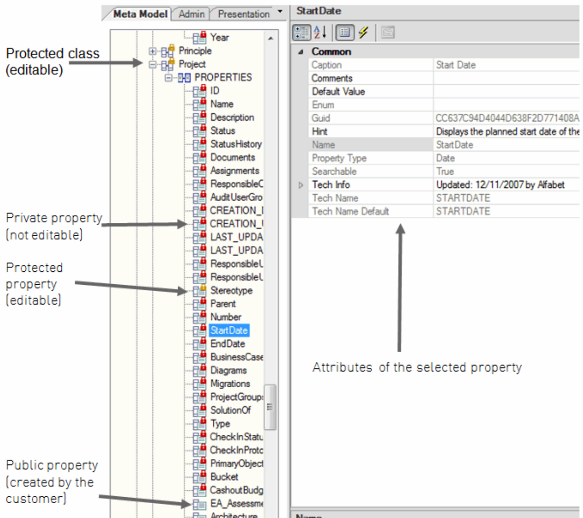
FIGURE: Attributes of the object class property StartDate of the object class Project displayed in the explorer of the tool Alfabet Expand
