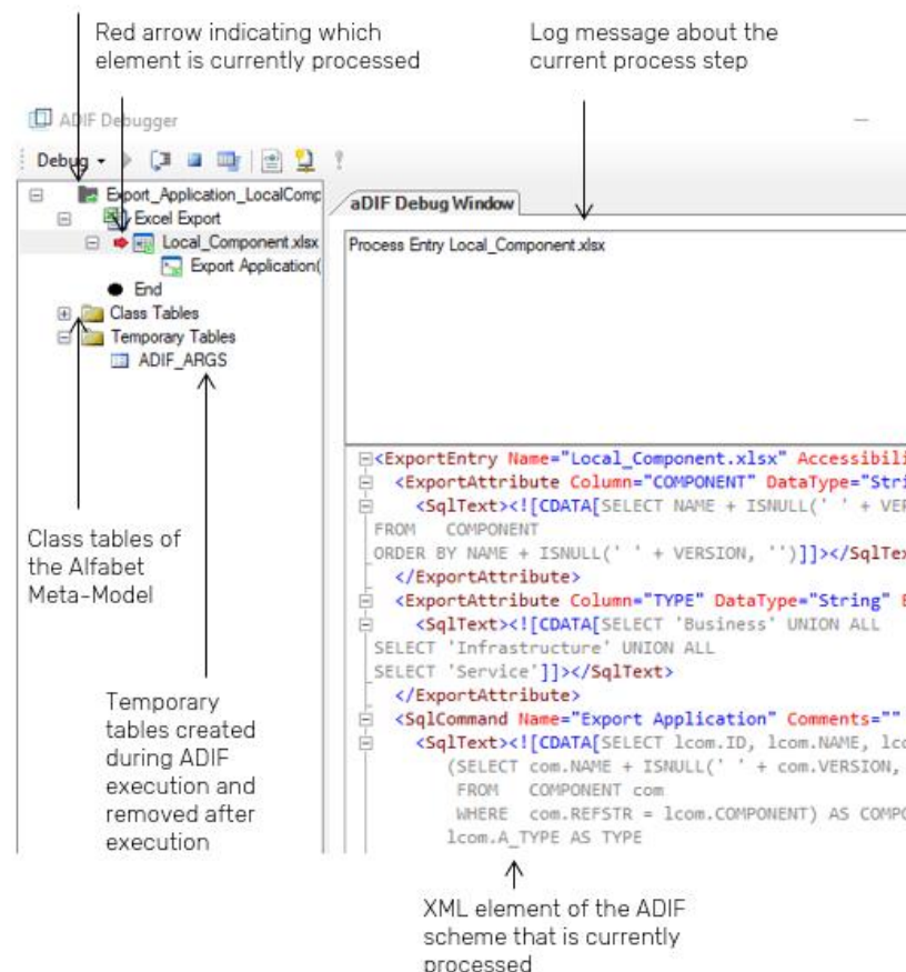
FIGURE: Interface of the ADIF Debugger
