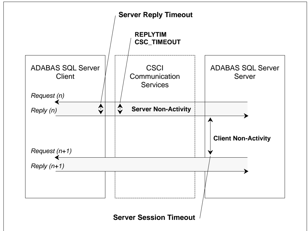
Figure 2-3: Client/server Time-Out Checking
