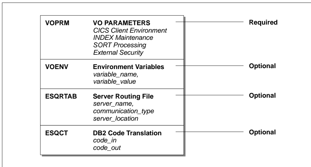
Figure 2-5: VOPRM Module Layout
