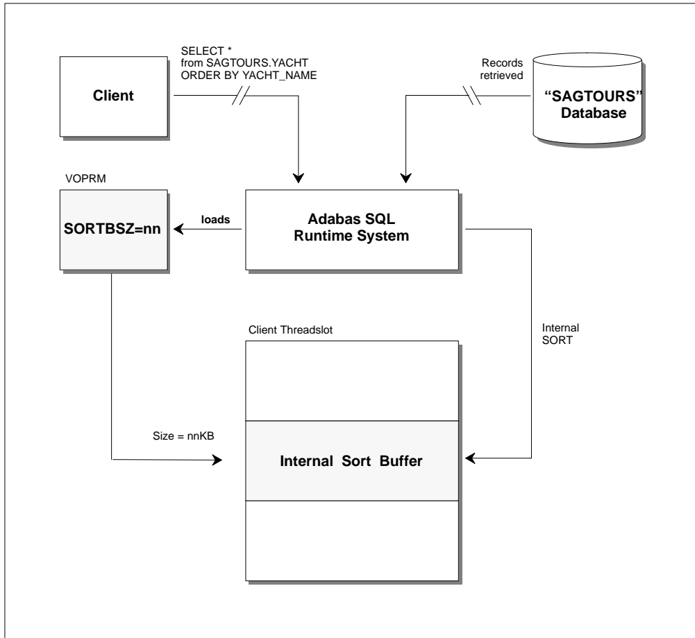
Figure 2-6: Internal SORT
