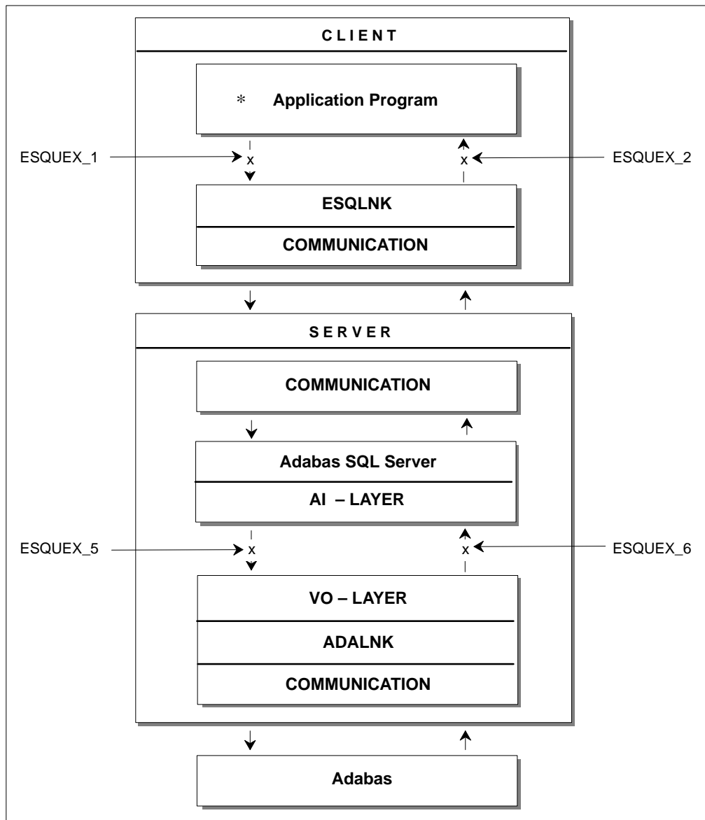
Figure 2-8: Locations of user exits within the Adabas SQL Server
