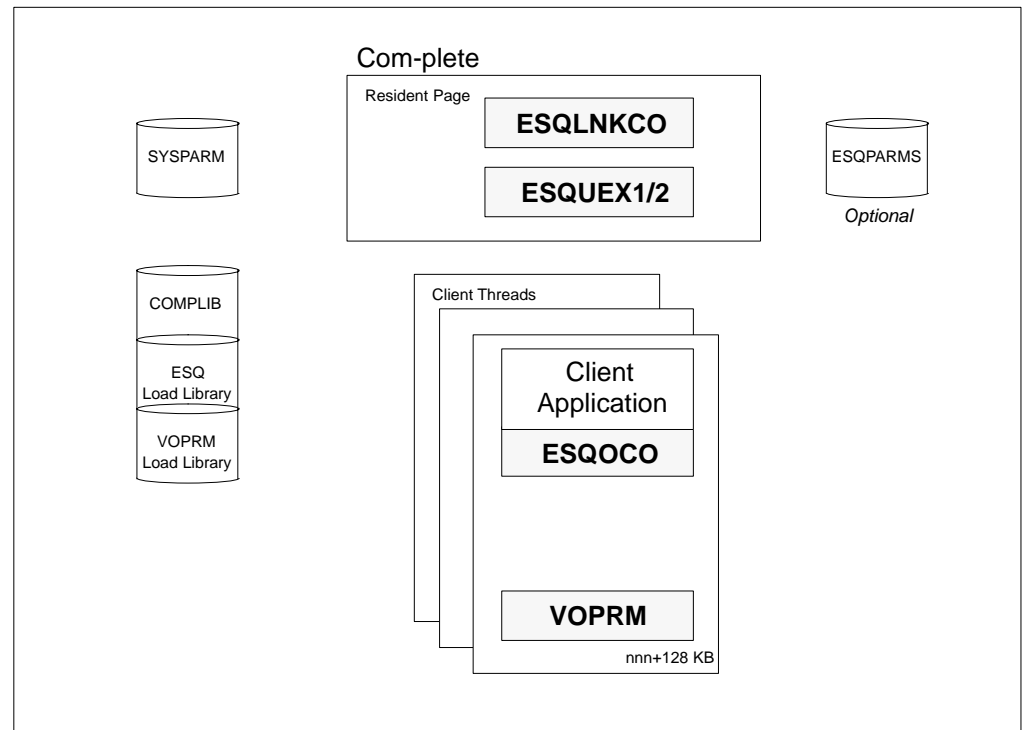
Figure 3-1: Adabas SQL Client under Com-plete
