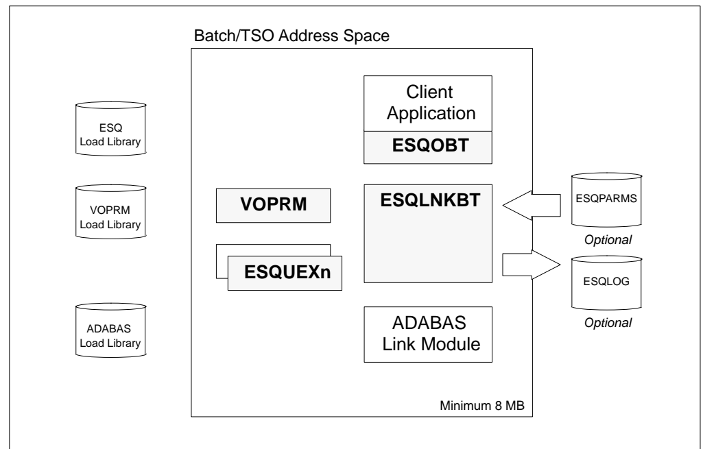
Figure 3-2: Adabas SQL Client under Batch/TSO
