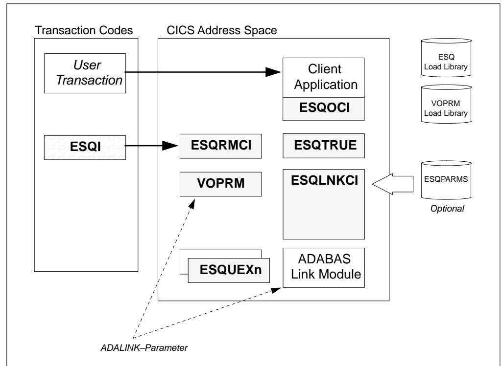
Figure 3-3: Adabas SQL Client under CICS
