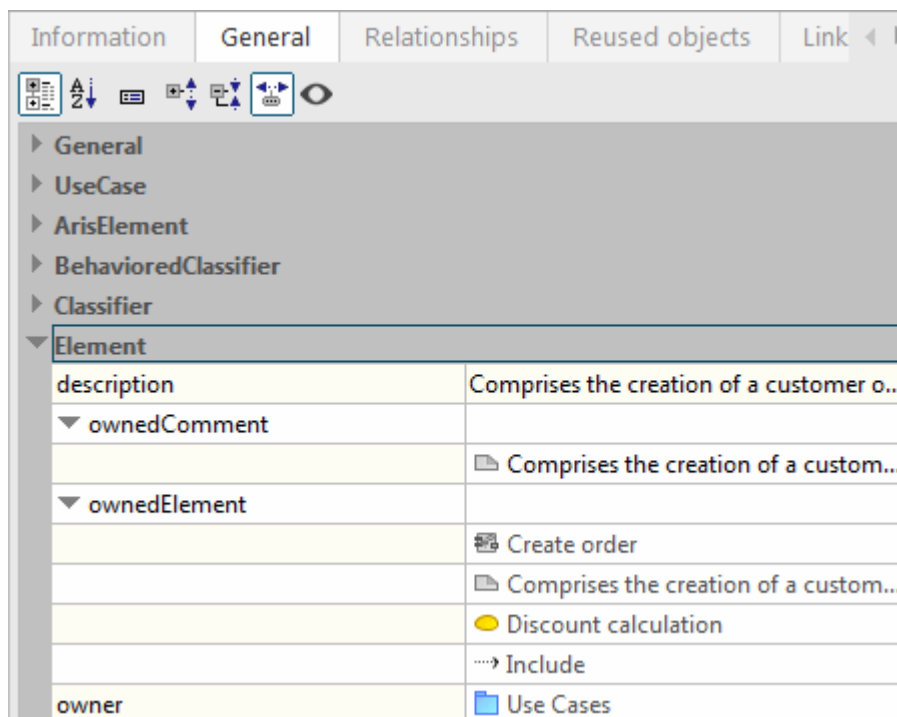
Figure 56: General properties page with display of derived properties
