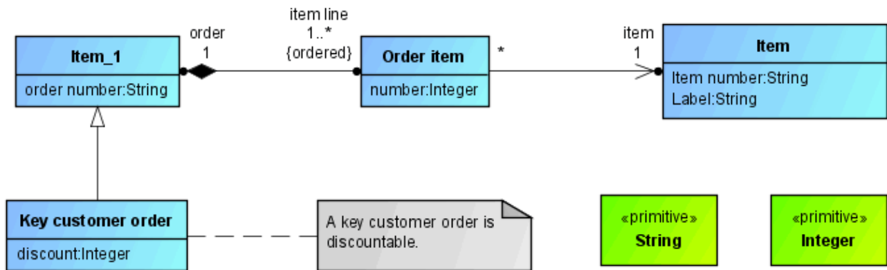
Figure 1: Class diagram
