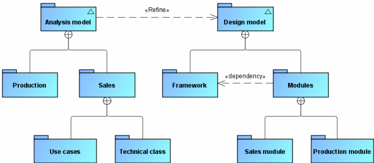
Figure 11: Package diagram
