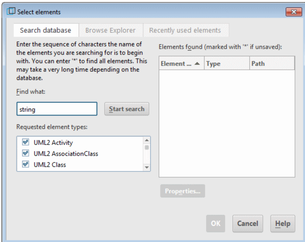
Figure 80: Search dialog
