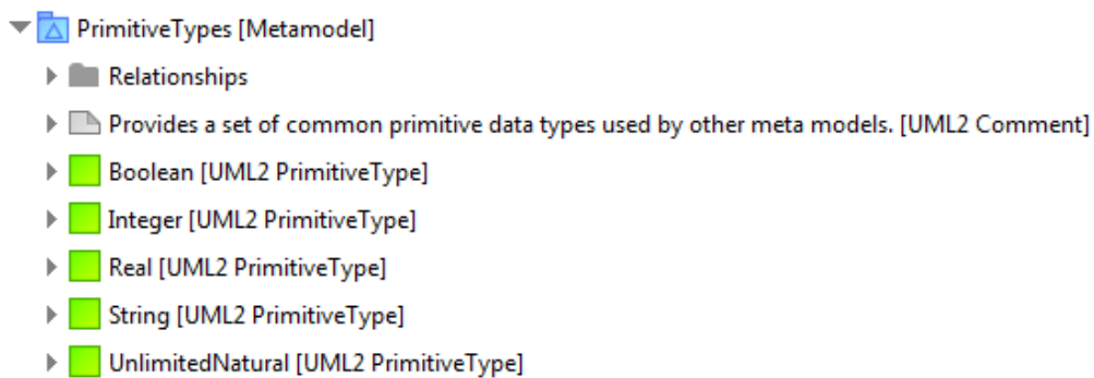
Figure 210: PrimitiveTypes metamodel
