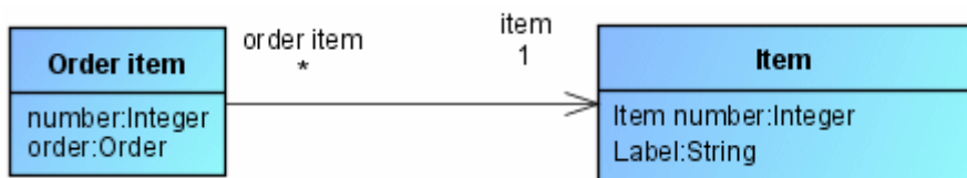
Figure 133: Association end navigable but not an attribute of the opposite class
