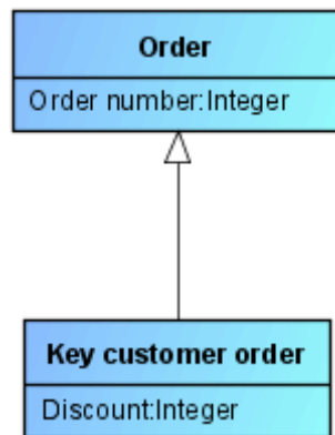
Figure 5: Generalization between two classes
