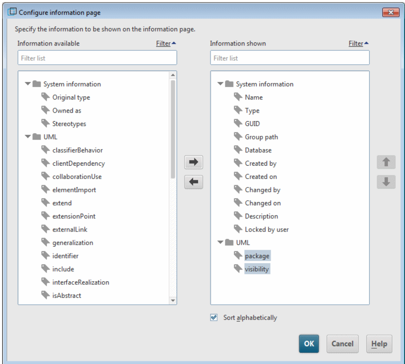
Figure 51: Information properties page configuration
