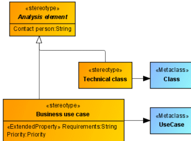
Figure 238: Inheritance relationships between stereotypes
