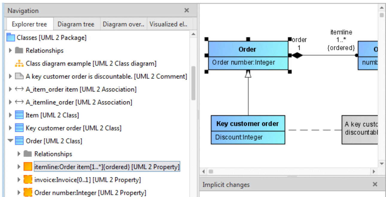
Figure 95: Binary associations whose ends are attributes of the classes involved
