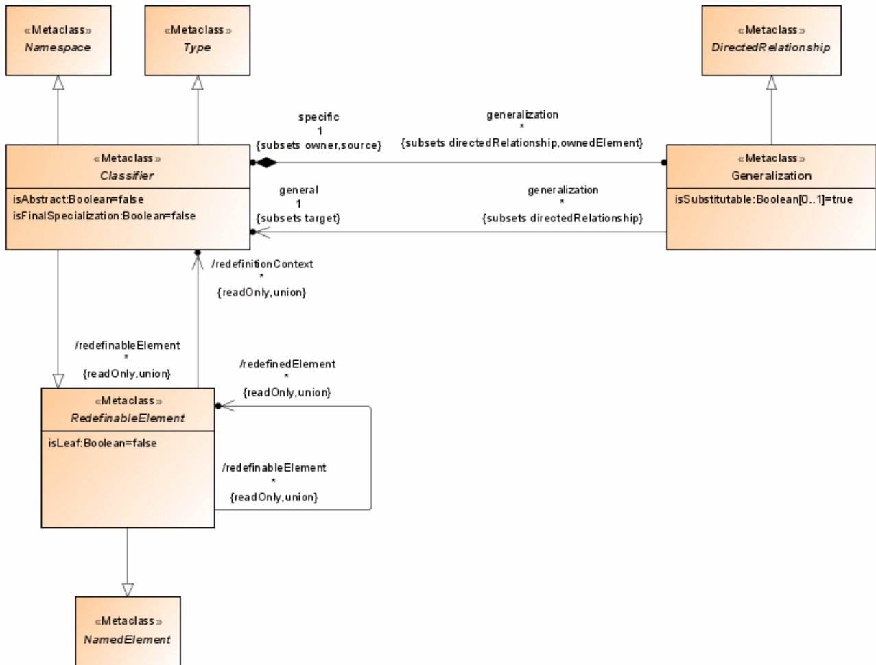
Figure 31: Classifiers diagram from the UML specification
