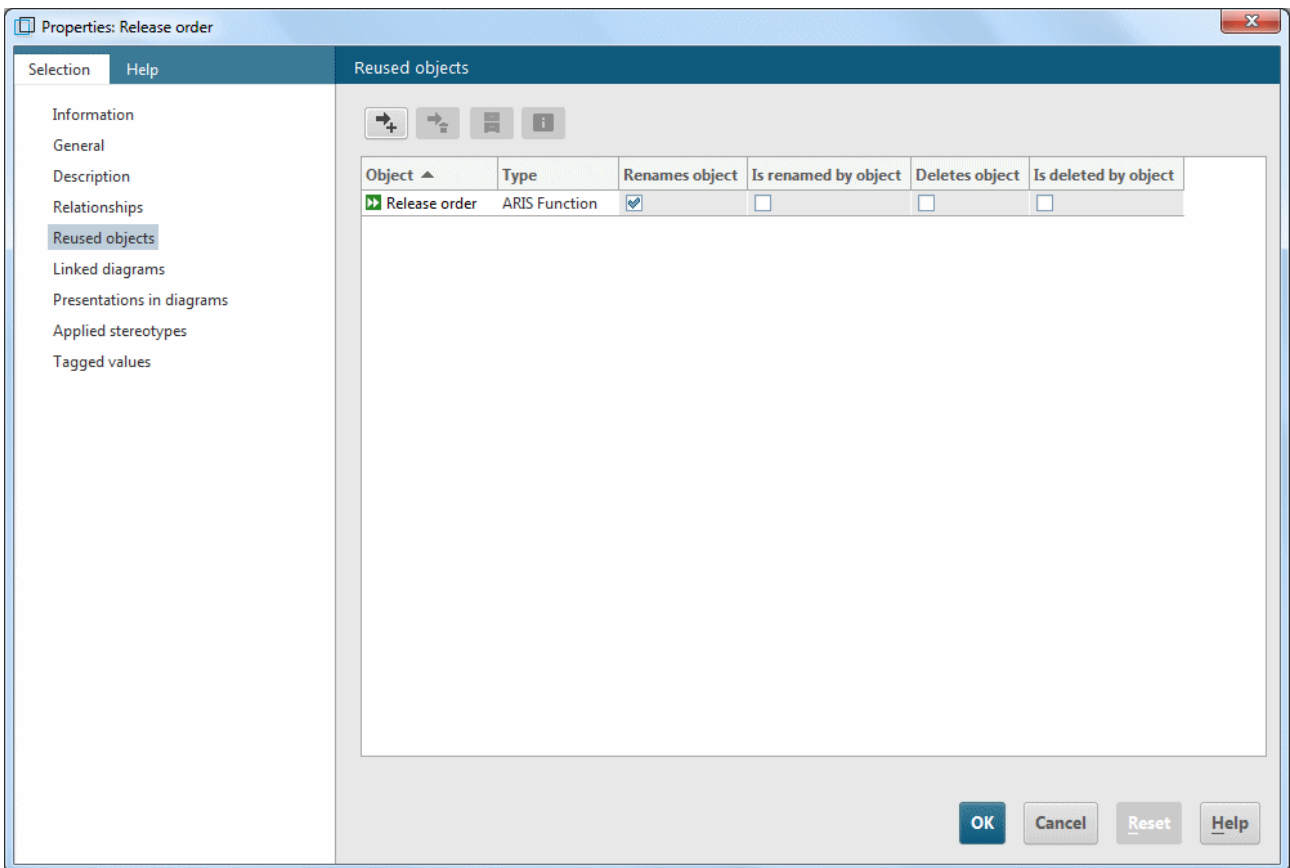
Figure 180: Reused objects properties page in ARIS UML Designer
