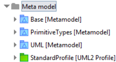
Figure 209: Generated metamodels
