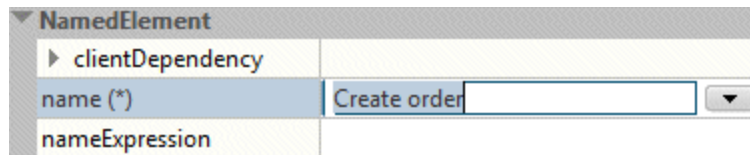
Figure 56: Text entry
