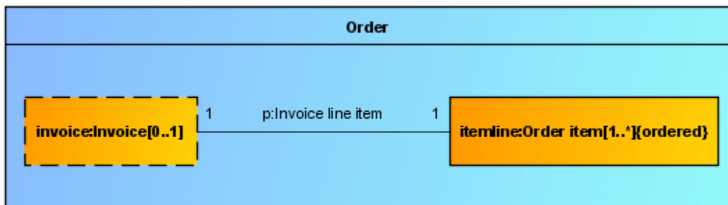
Figure 9: Composite structure diagram for the Order class
