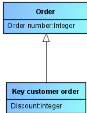
Figure 32: Generalization relationship between two classes
