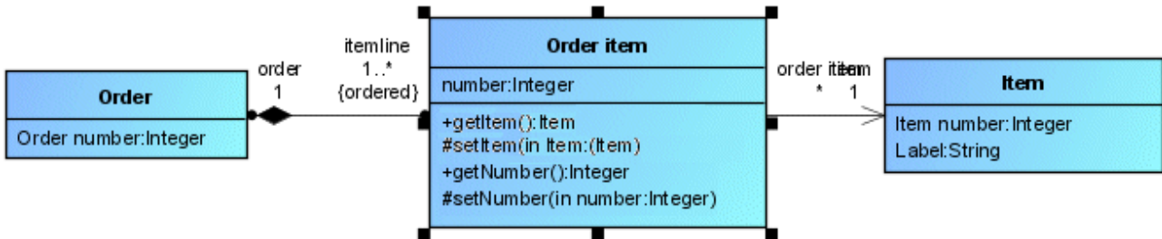
Figure 137: Generated getters and setters
