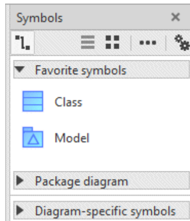
Figure 91: Favorite symbols
