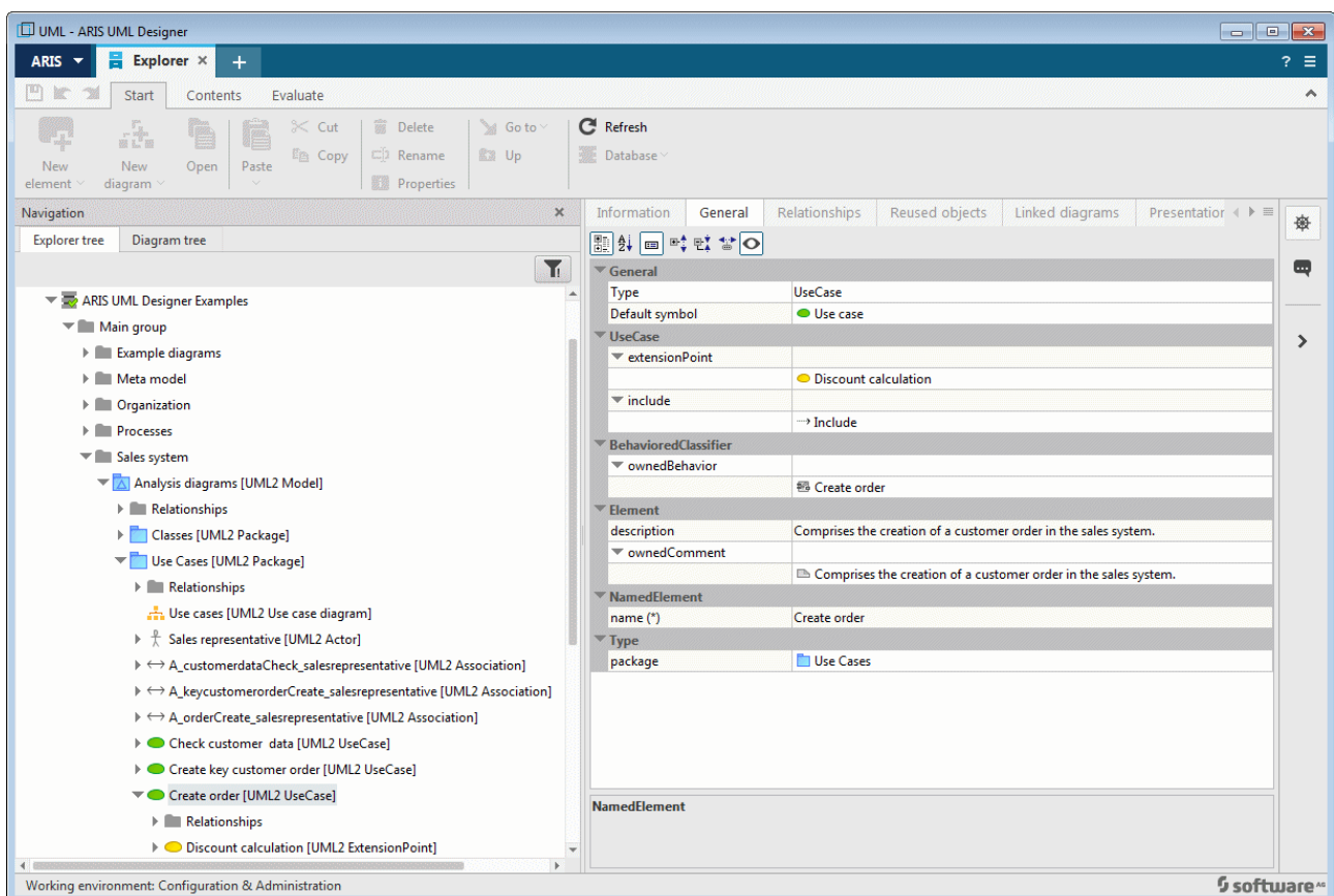
Figure 43: Explorer tab
