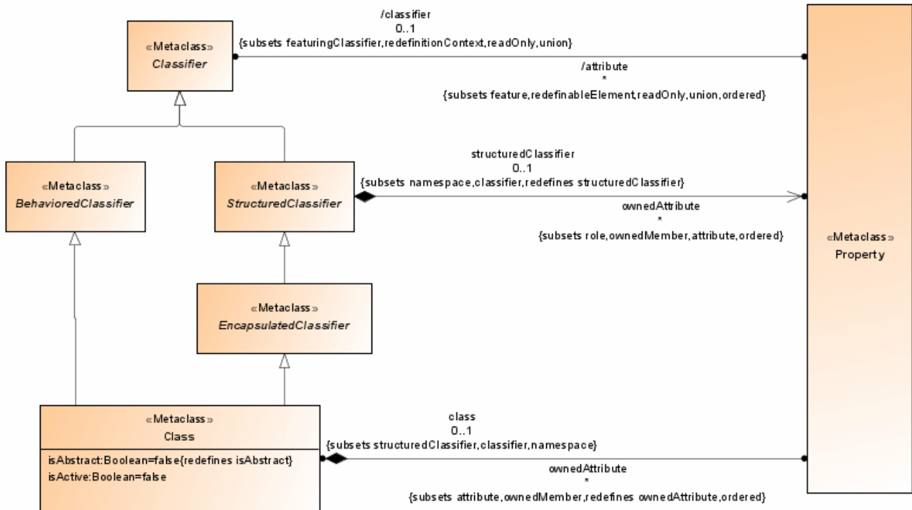
Figure 35: Classes diagram from the UML specification
