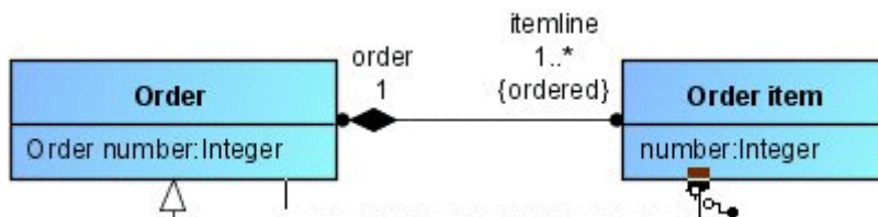
Figure 105: Displaying the edge anchor point on the target element and edge preview
