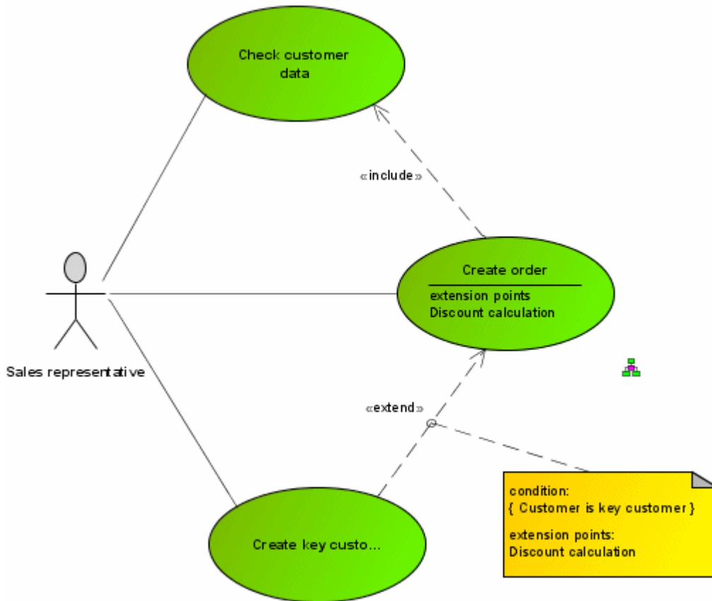
Figure 17: Use case diagram
