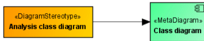
Figure 243: Definition of a stereotype for class diagrams
