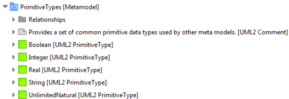
Figure 210: PrimitiveTypes metamodel
