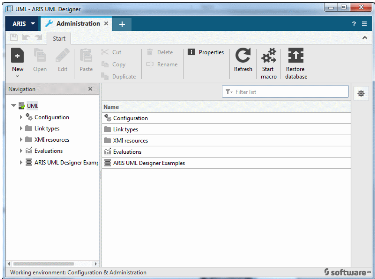
Figure 153: Administration component
