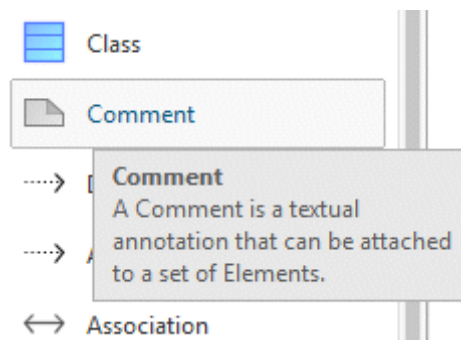
Figure 85: Symbol description
