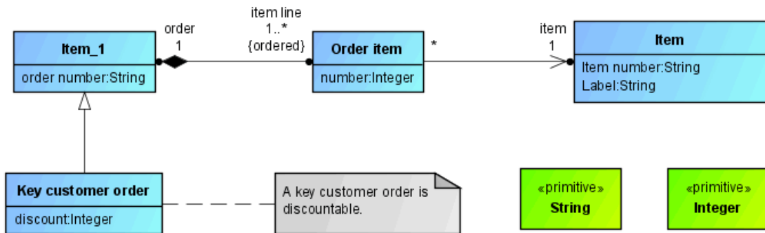
Figure 1: Class diagram
