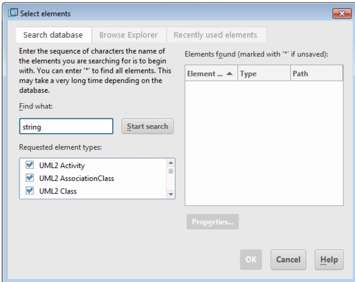
Figure 78: Search dialog
