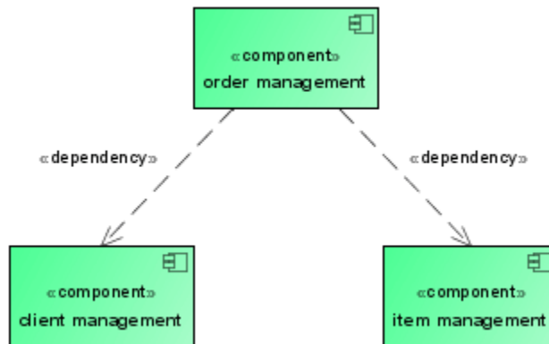
Figure 6: Component diagram
