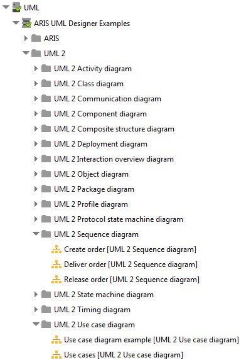
Figure 49: Diagram tree
