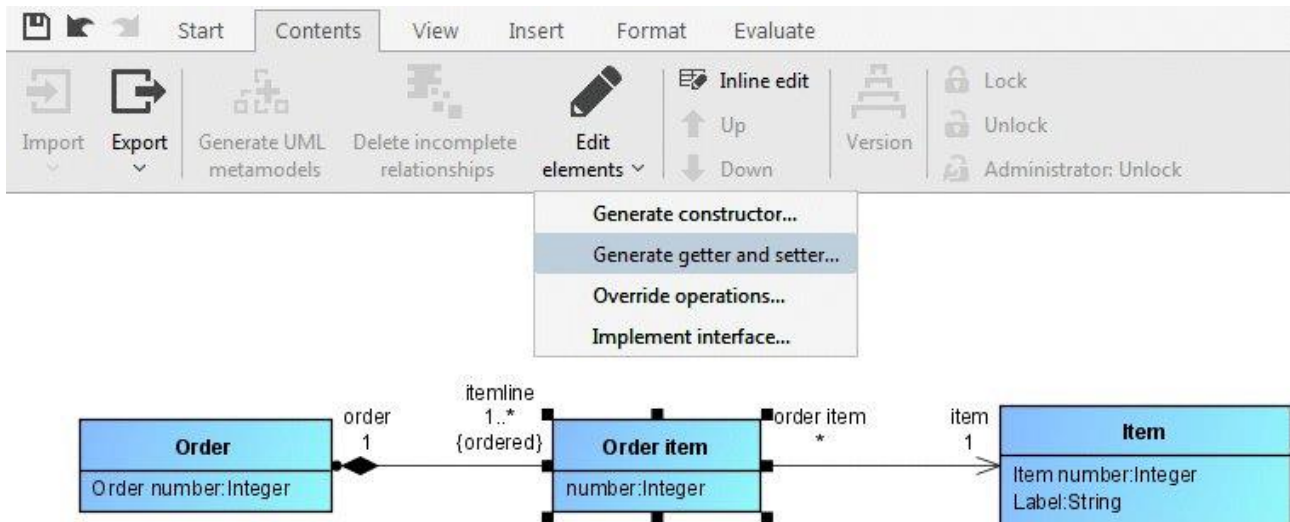
Figure 135: Functionalities for creating operations for a class
