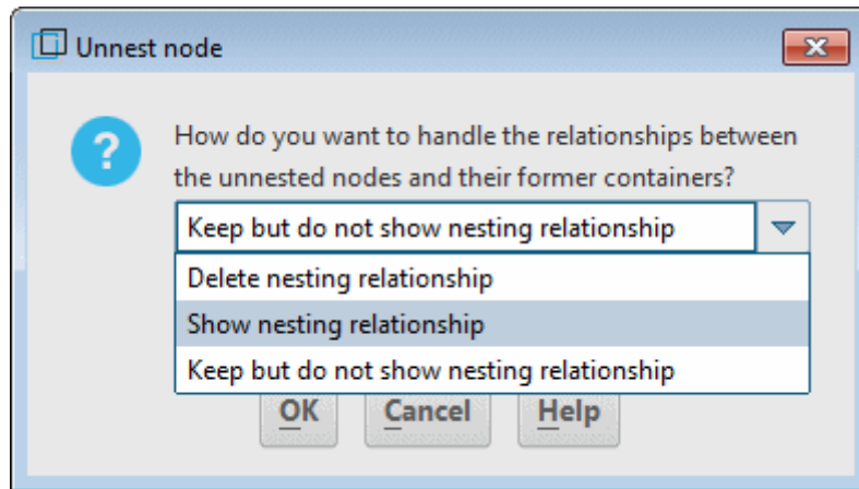
Figure 118: Unnest node dialog
