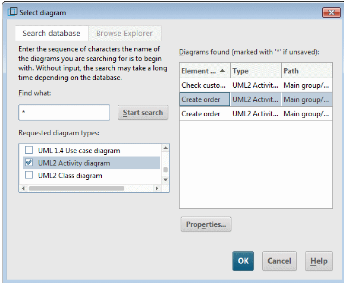
Figure 161: Diagram selection by searching in the database
