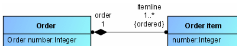
Figure 34: Class diagram with attributes and association ends
