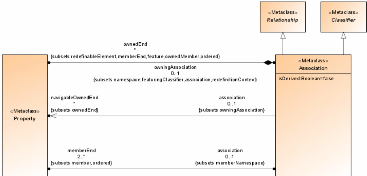
Figure 36: Associations diagram from the UML specification
