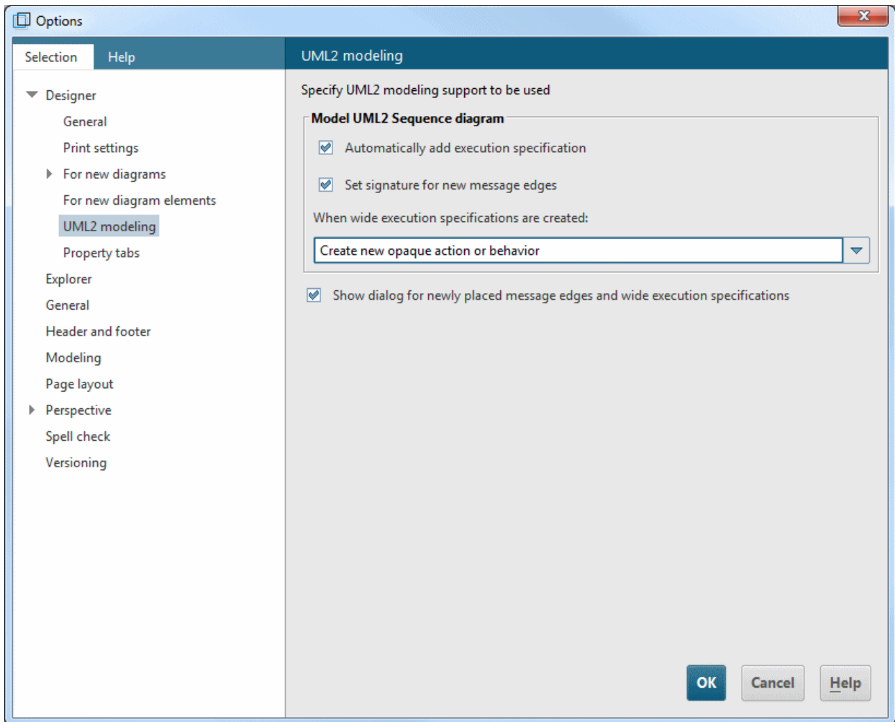
Figure 151: Designer > UML2 Modeling options page
