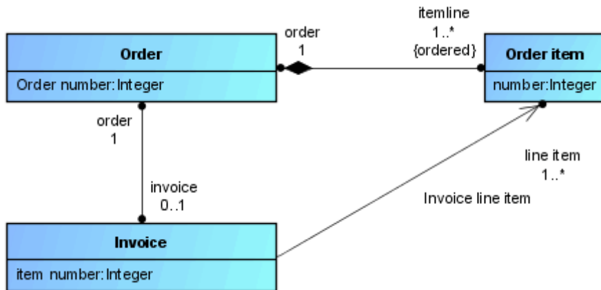
Figure 8: Class diagram with order components
