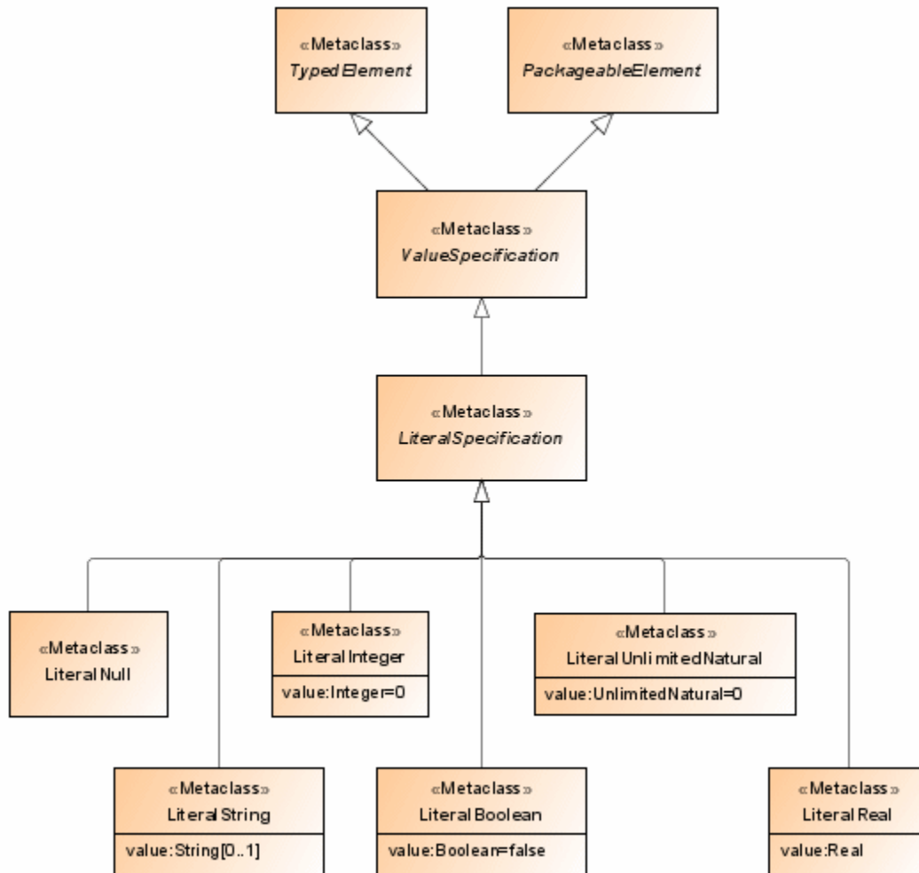
Figure 187: Literals diagram from the UML specification
