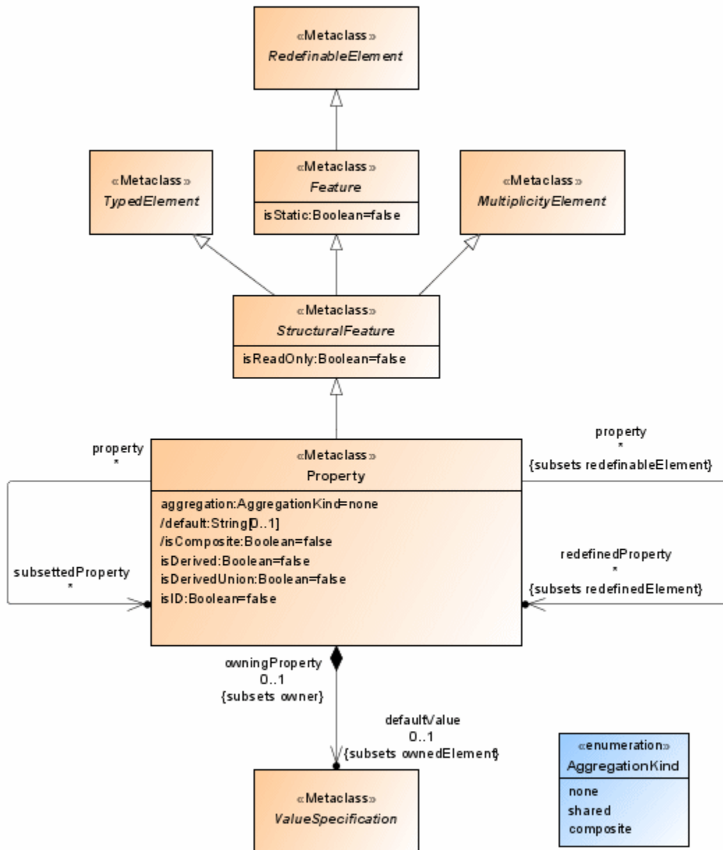
Figure 33: Features diagram from the UML specification
