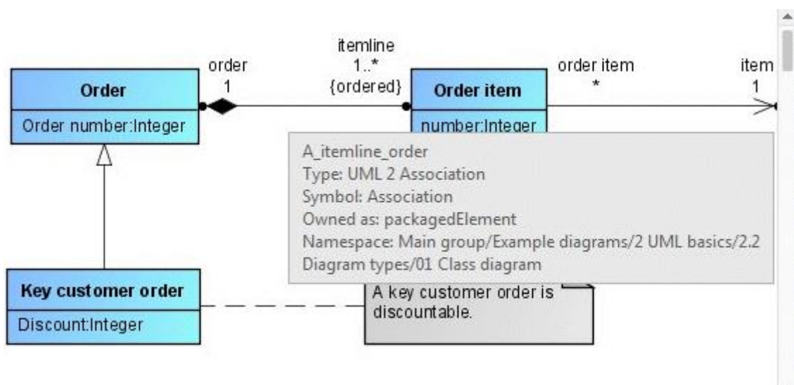
Figure 159: Association as graphic edge in diagram
