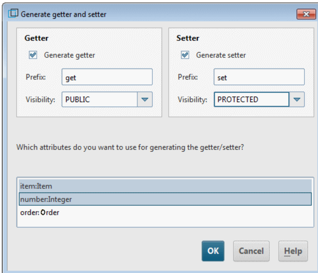
Figure 136: Generate getter and setter dialog
