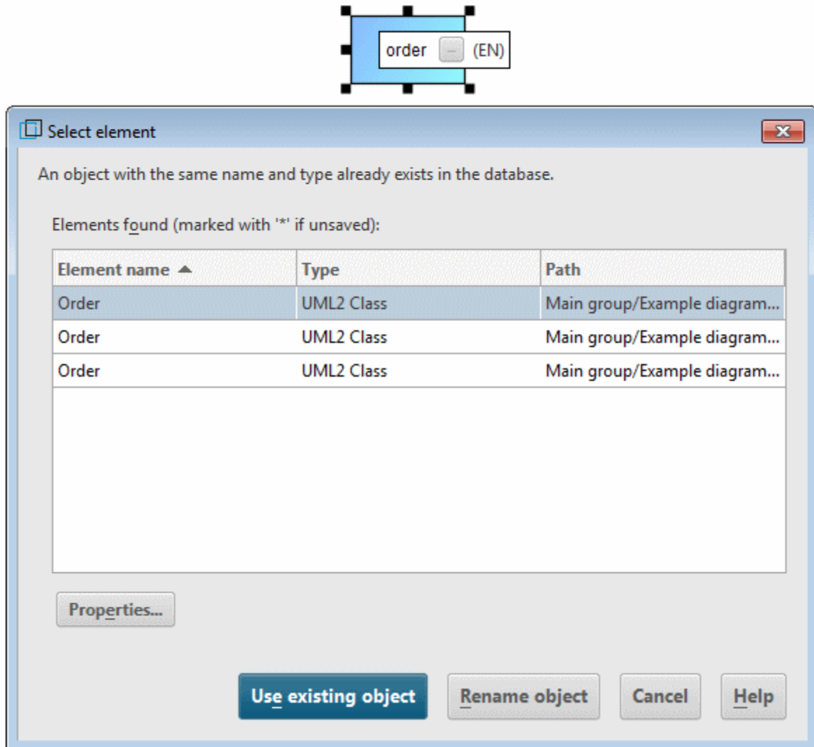
Figure 101: Create dialog after entering the name of existing elements
