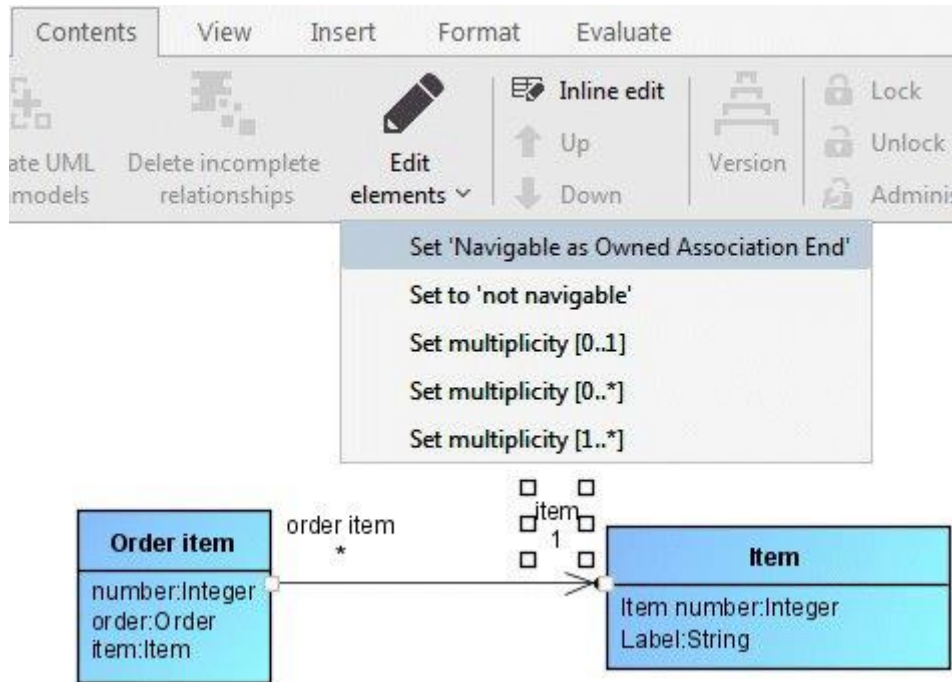
Figure 132: Functions for changing the navigability and the multiplicity
