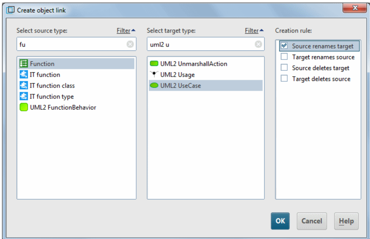
Figure 171: Definition of a mapping of the ARIS object type Function to the UML 2 element type UseCase
