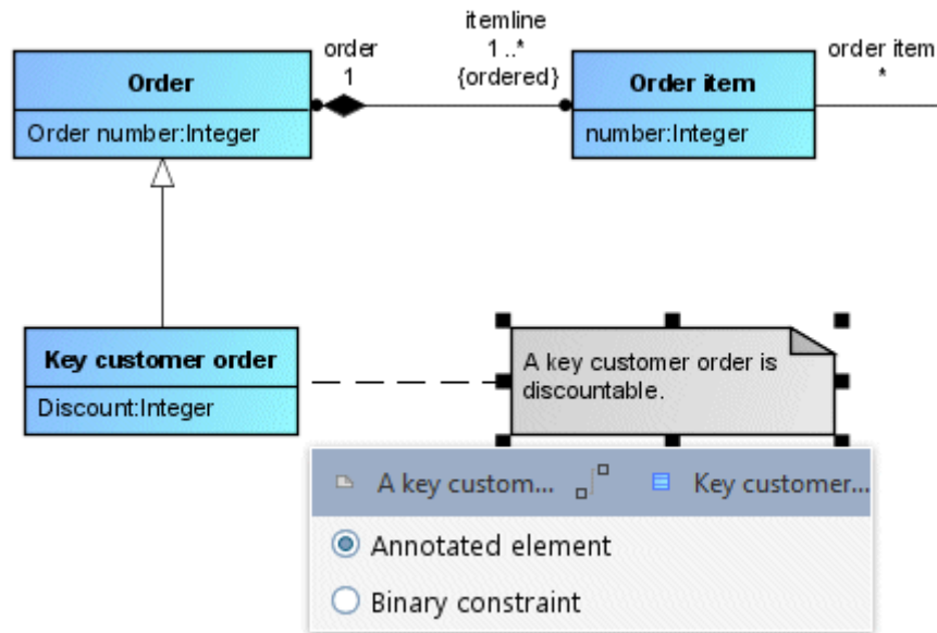
Figure 111: Node and edge preview with edge type selection after clicking the Comment symbol in the mini toolbar
