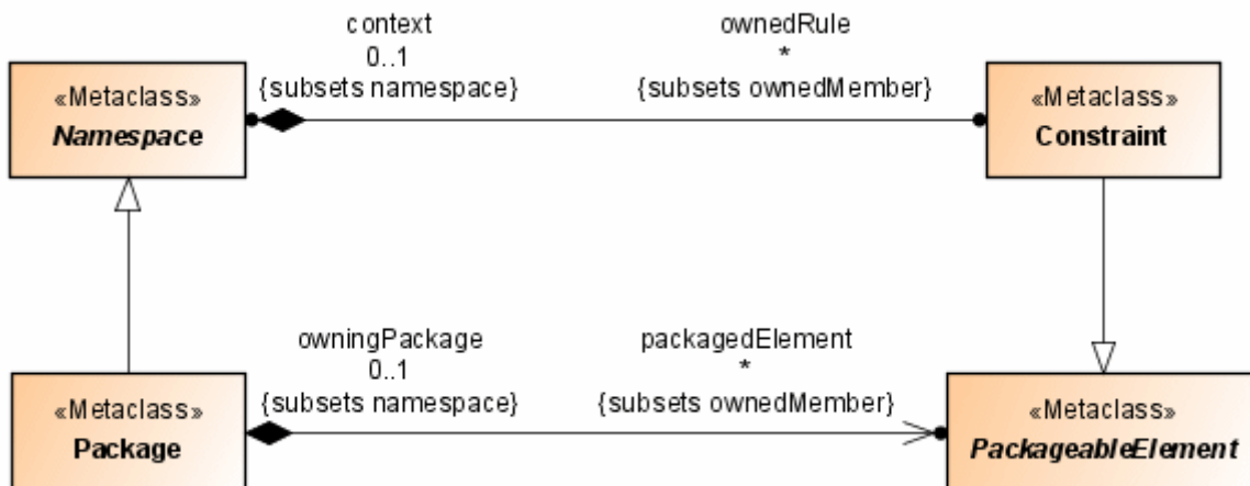
Figure 120: Extract from the UML metamodel with the Package and Constraint metaclasses
