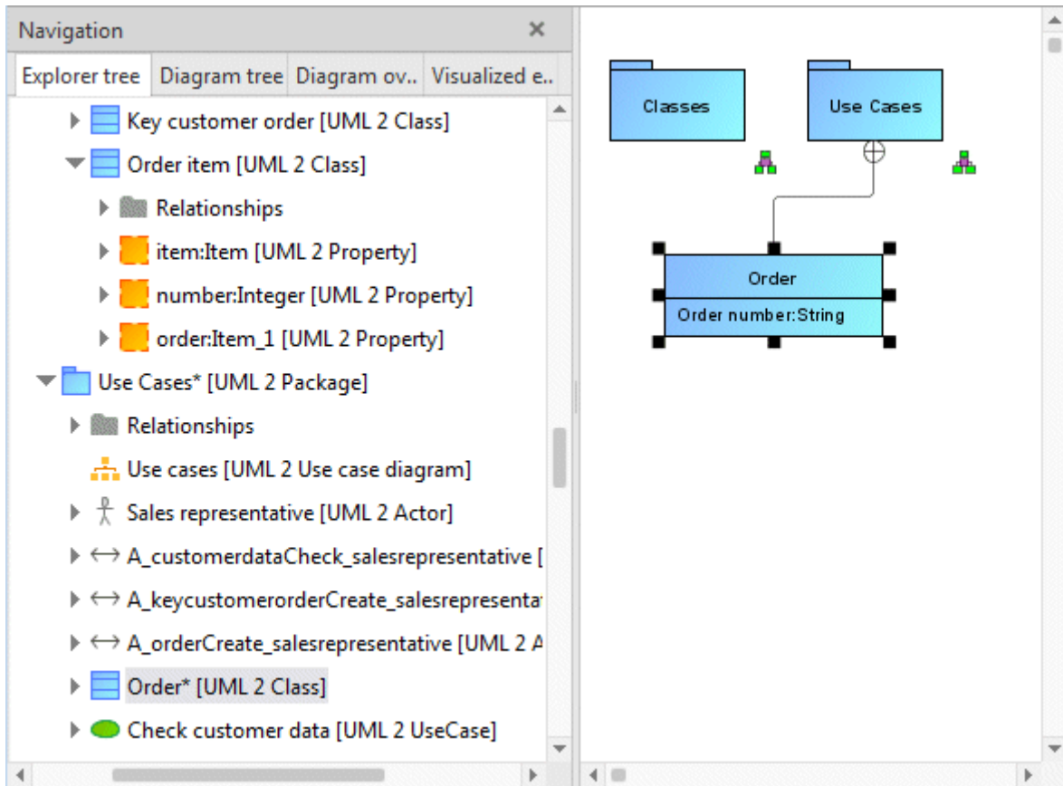
Figure 114: After creating a second owning package relationship
