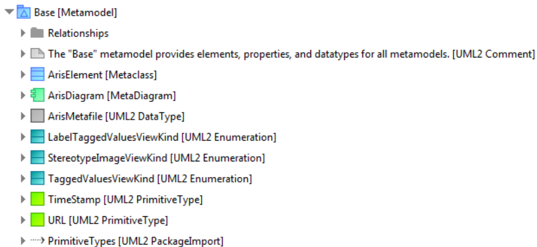
Figure 211: Base metamodel
