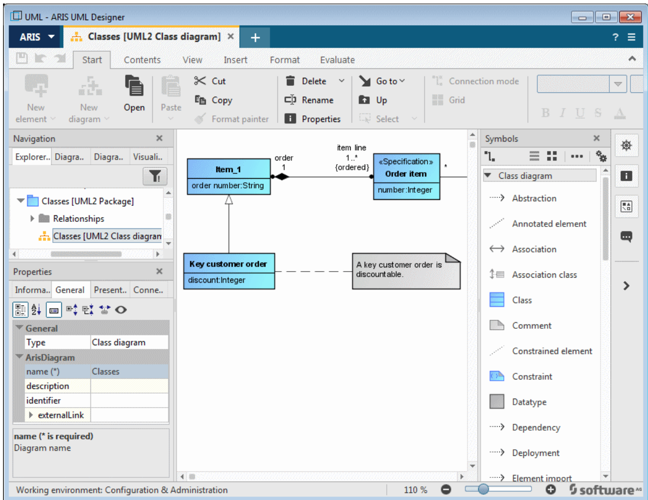
Figure 80: Designer component
