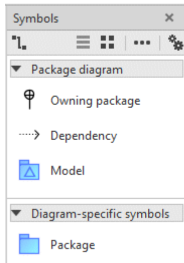
Figure 93: Diagram-specific symbols
