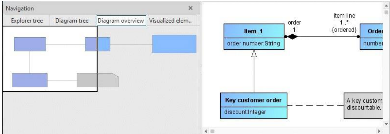
Figure 81: Diagram overview
