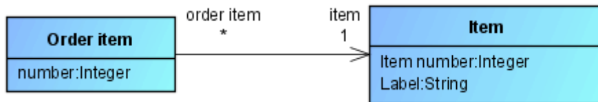
Figure 4: Unidirectional association
