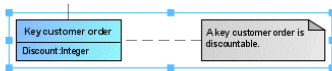
Figure 127: Grouped elements
