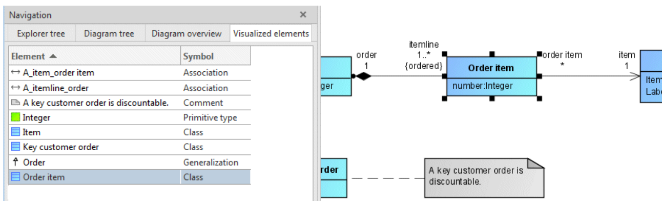
Figure 82: Visualized elements
