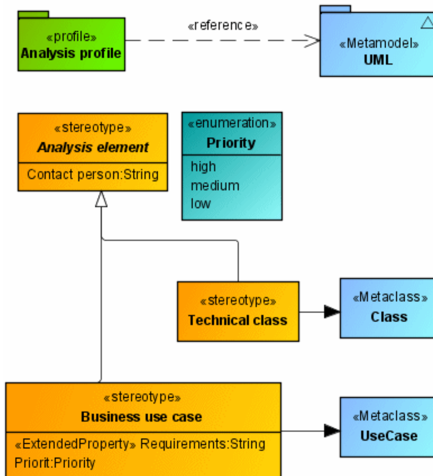
Figure 12: Profile diagram
