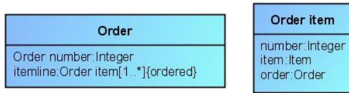
Figure 3: Association ends as attributes
