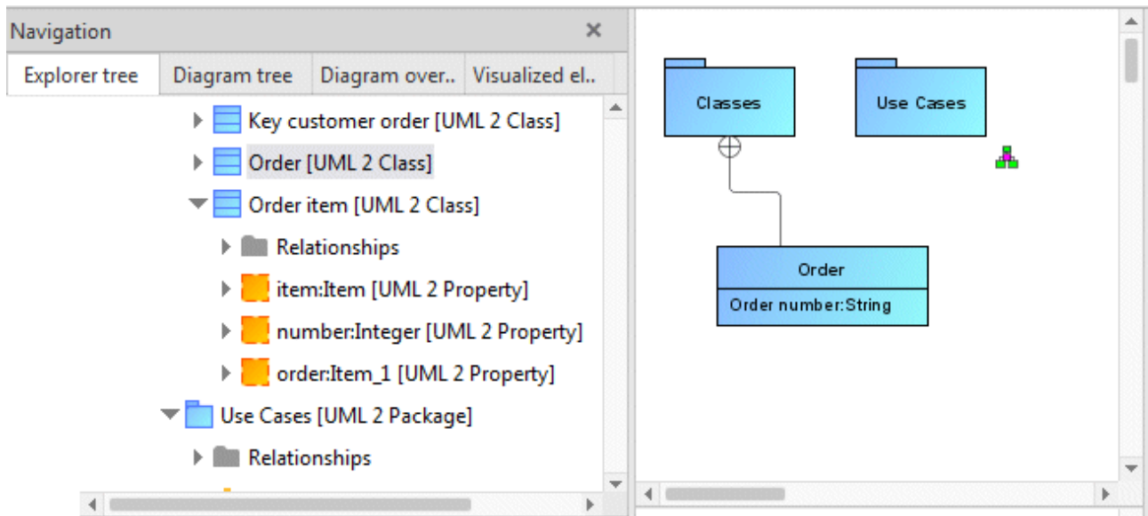
Figure 113: Owning package relationship between a class and the package in which it is contained
