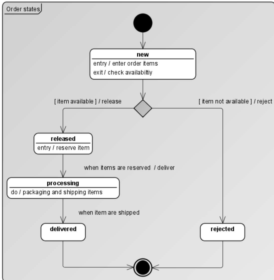
Figure 22: Order states state machine diagram
