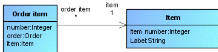
Figure 130: Unidirectional navigable association
