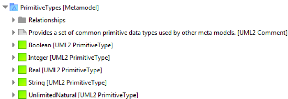
Figure 210: PrimitiveTypes metamodel
