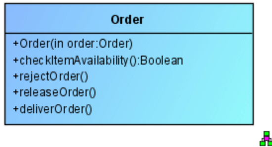
Figure 23: Order class with operations
