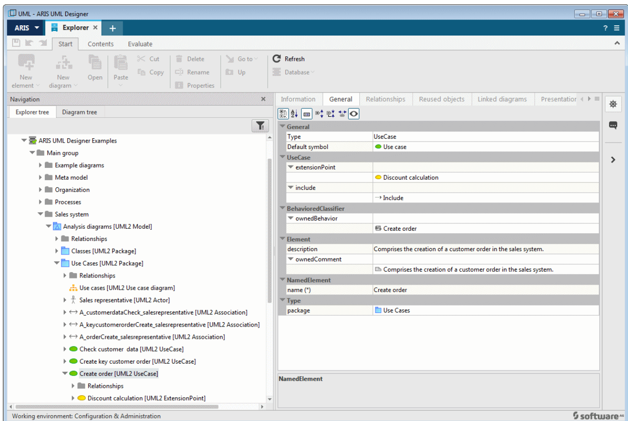
Figure 43: Explorer tab
