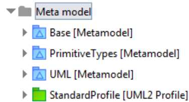
Figure 209: Generated metamodels
