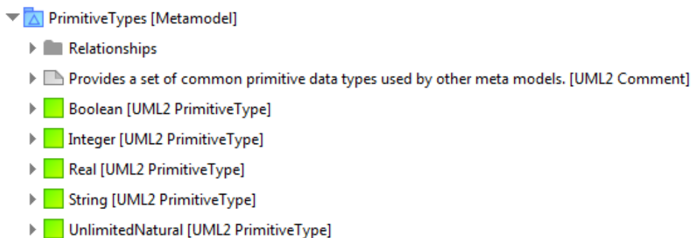
Figure 210: PrimitiveTypes metamodel
