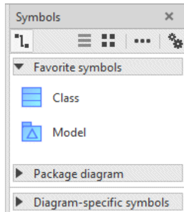
Figure 91: Favorite symbols
