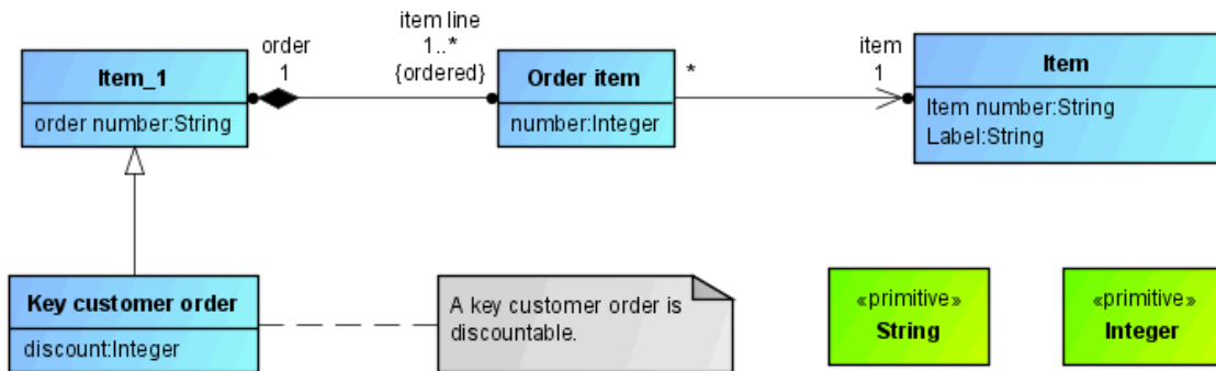
Figure 1: Class diagram
