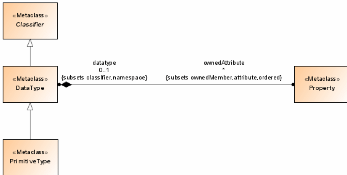
Figure 38: DataTypes diagram from the UML specification
